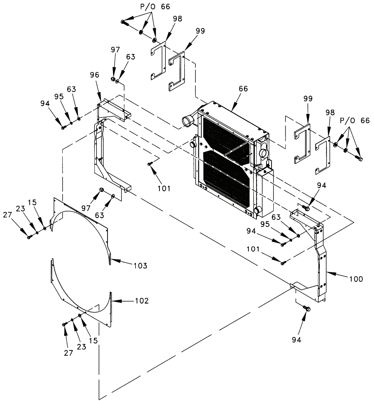
Figure 13. Cooling System Installation (Sheet 6 of 6).
