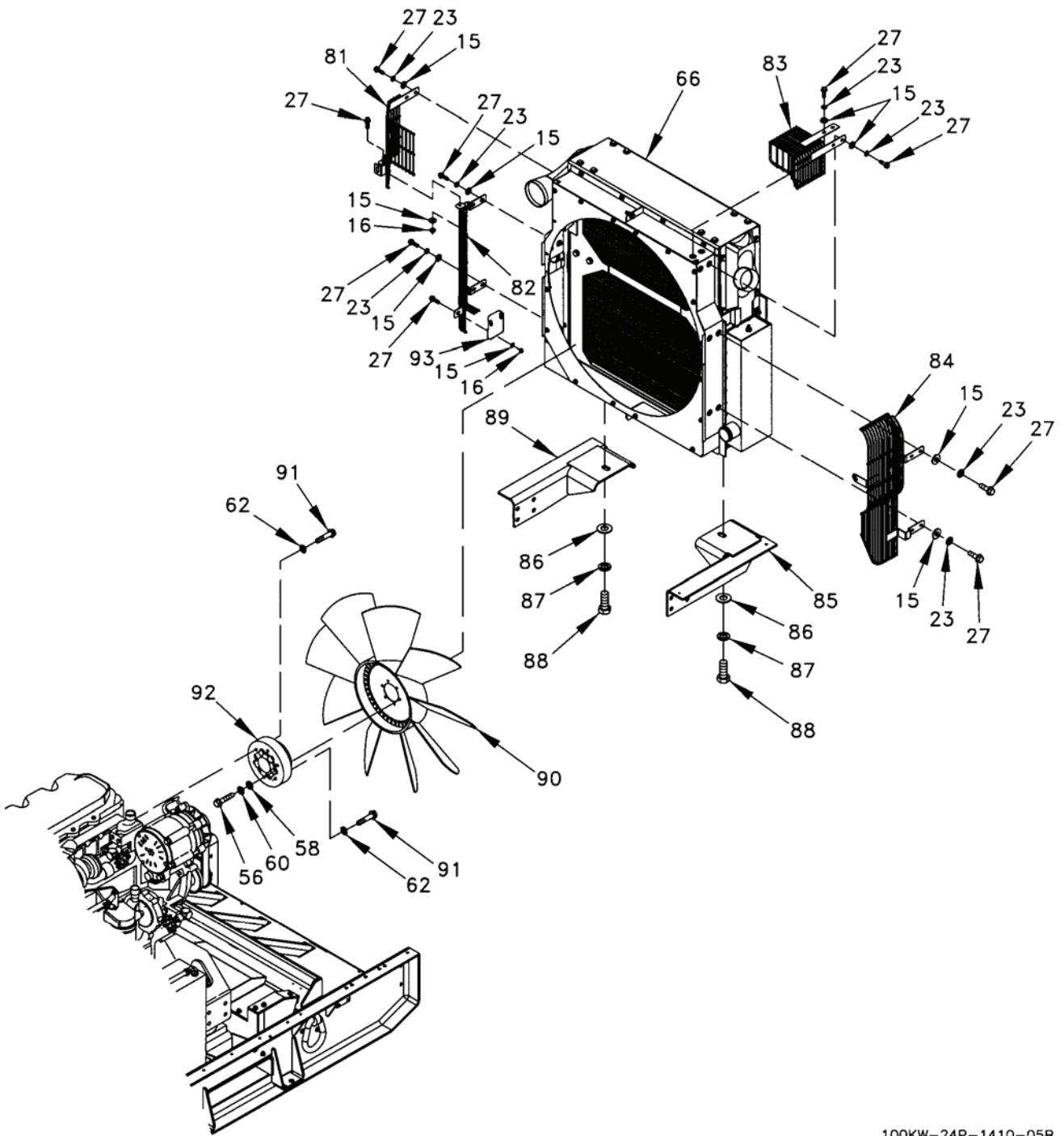
Figure 13. Cooling System Installation (Sheet 5 of 6).
