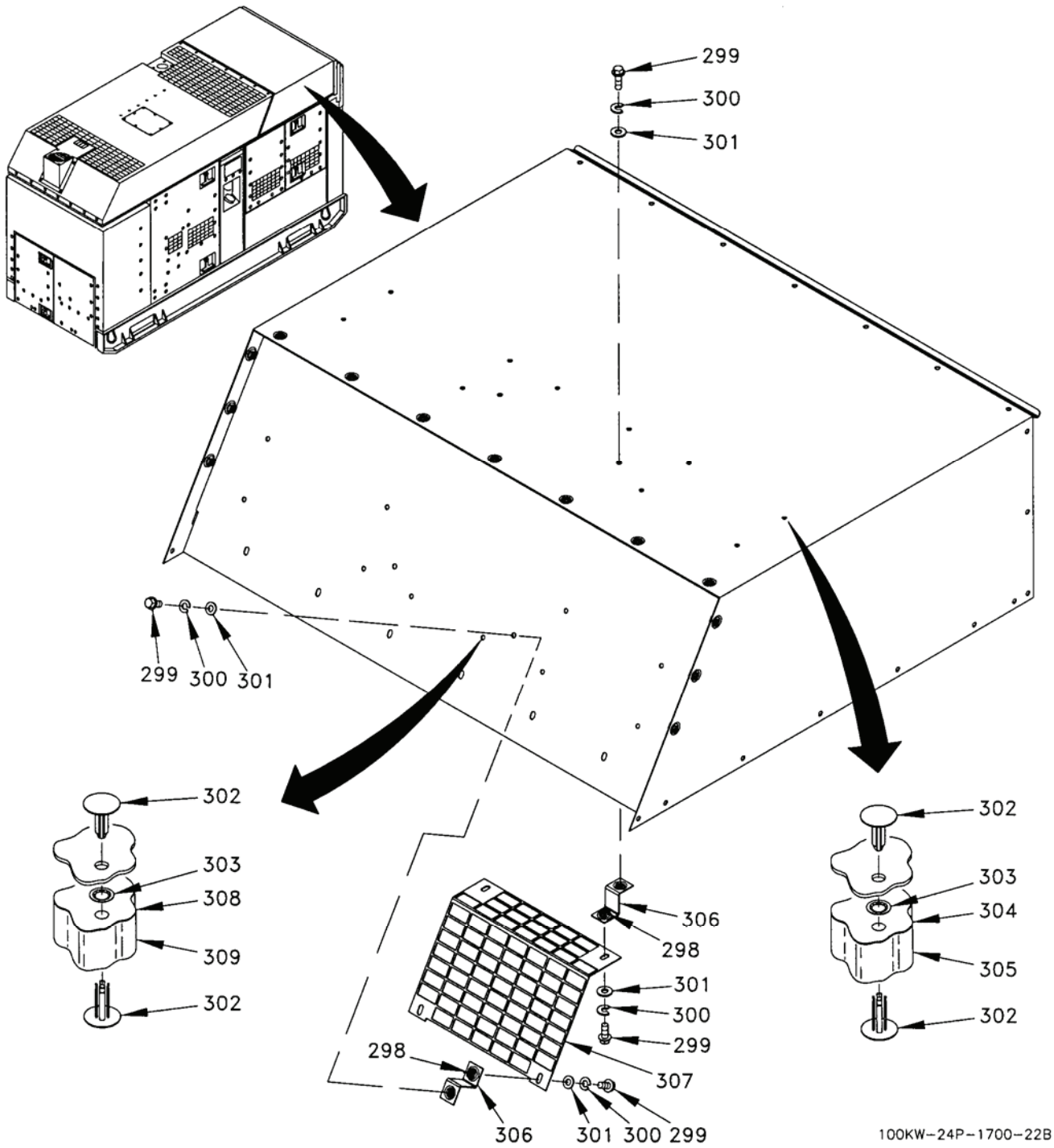
Figure 3. Housing Installation (Sheet 22 of 25).
