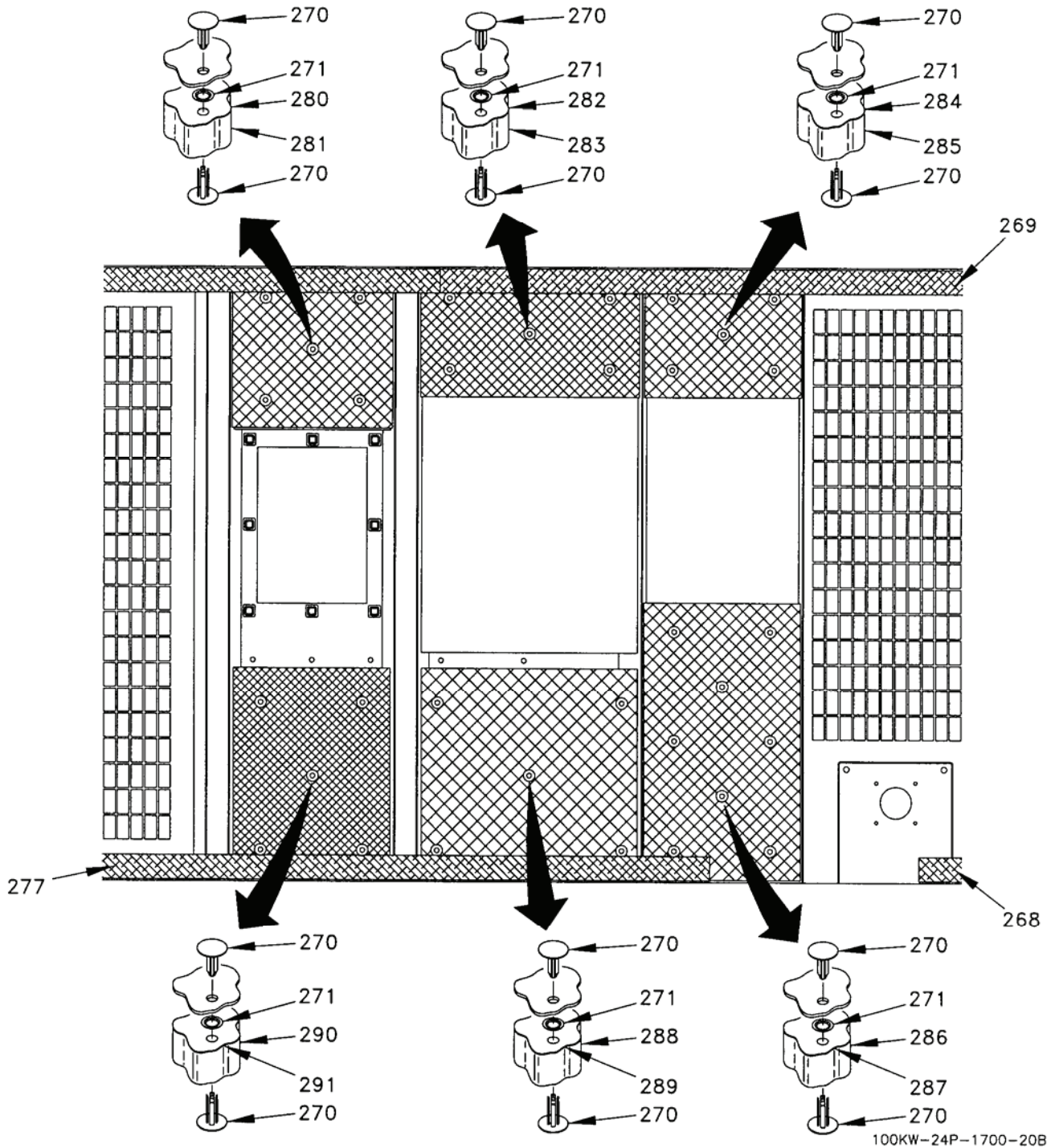
Figure 3. Housing Installation (Sheet 20 of 25).
