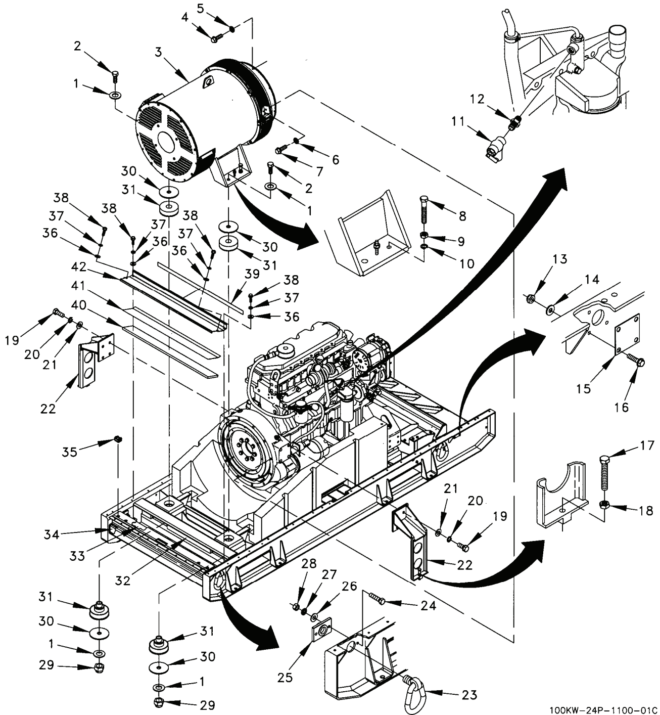
Figure 16. Engine Generator Base Assembly (Sheet 1 of 4).
