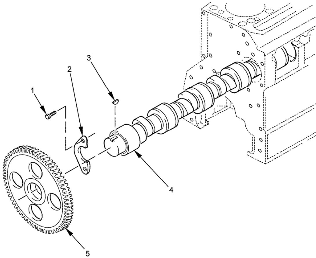
Figure 41. Camshaft Group.
