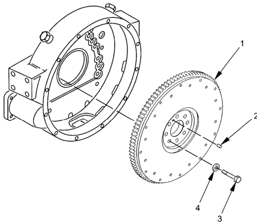
Figure 42. Flywheel Group.
