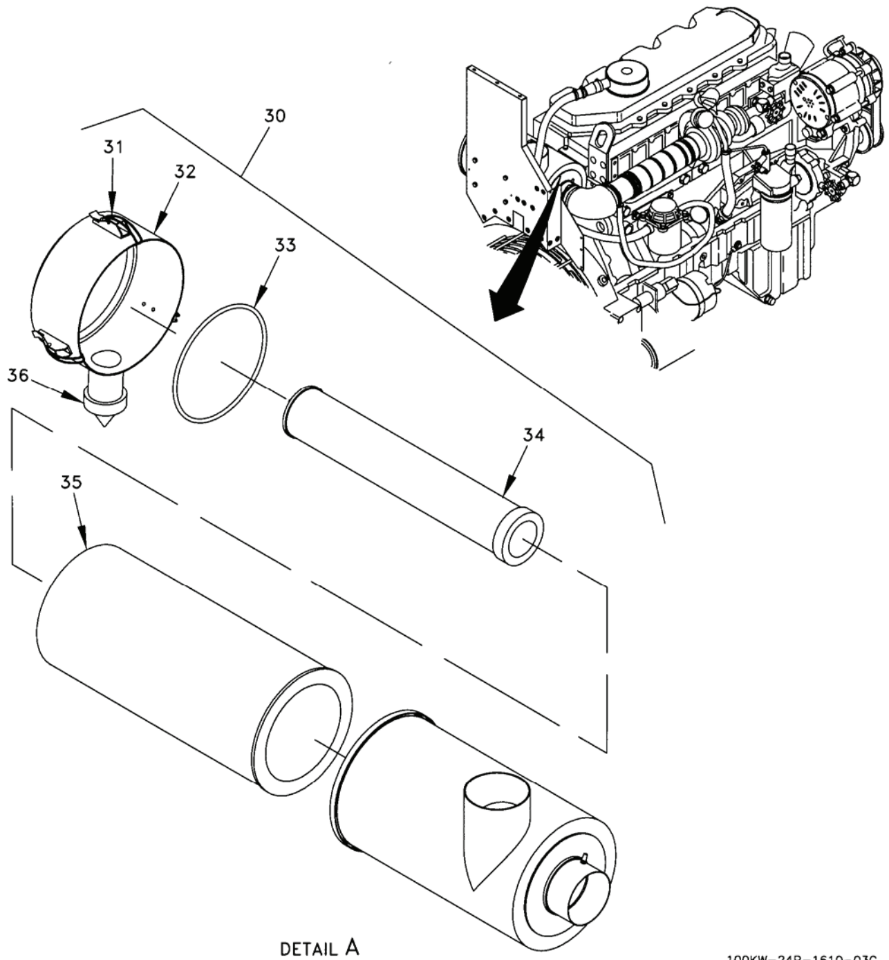
Figure 15. Air Cleaner Installation (Sheet 3 of 3).
