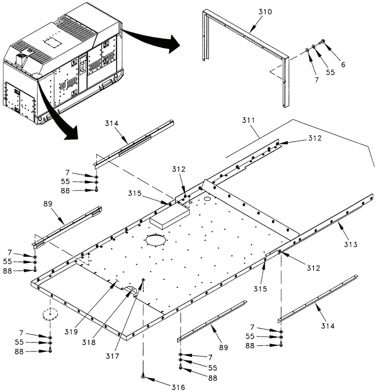
Figure 3. Housing Installation (Sheet 23 of 25).
