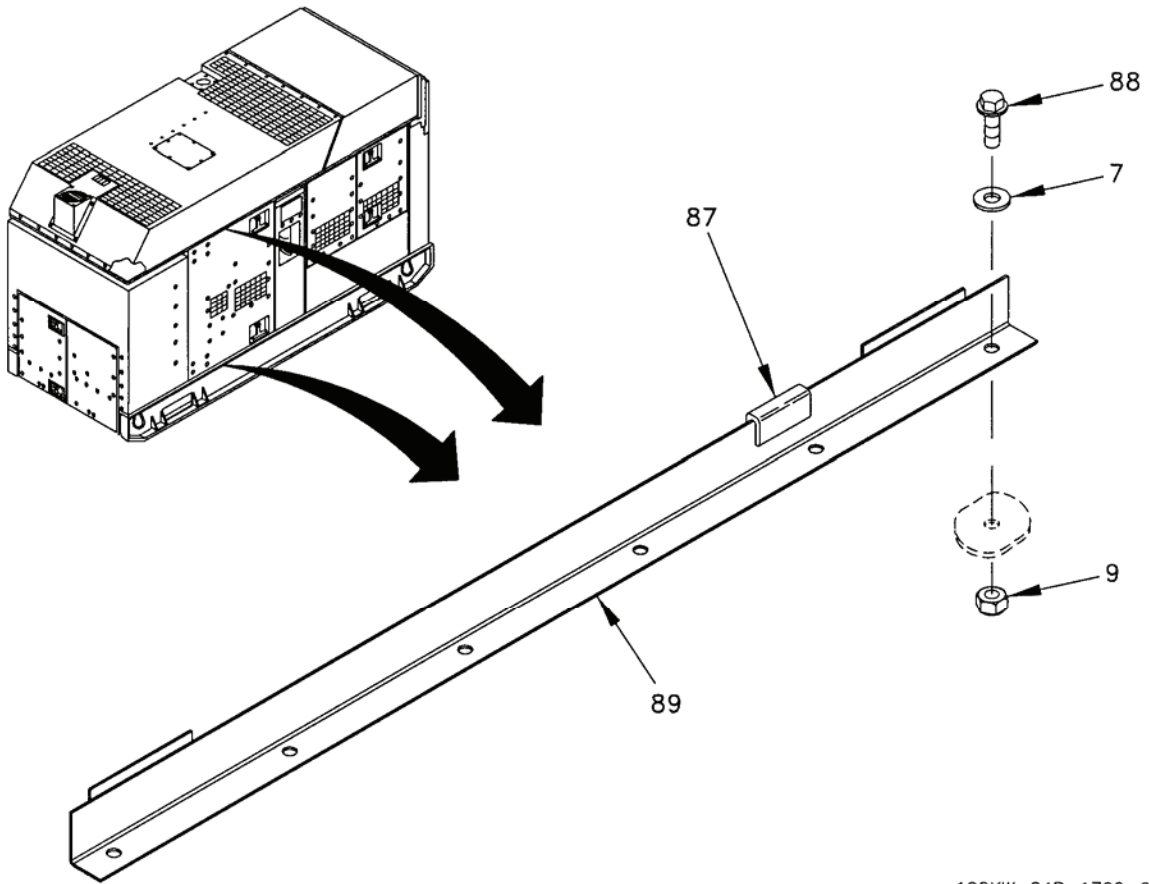
Figure 3. Housing Installation (Sheet 4 of 25).
