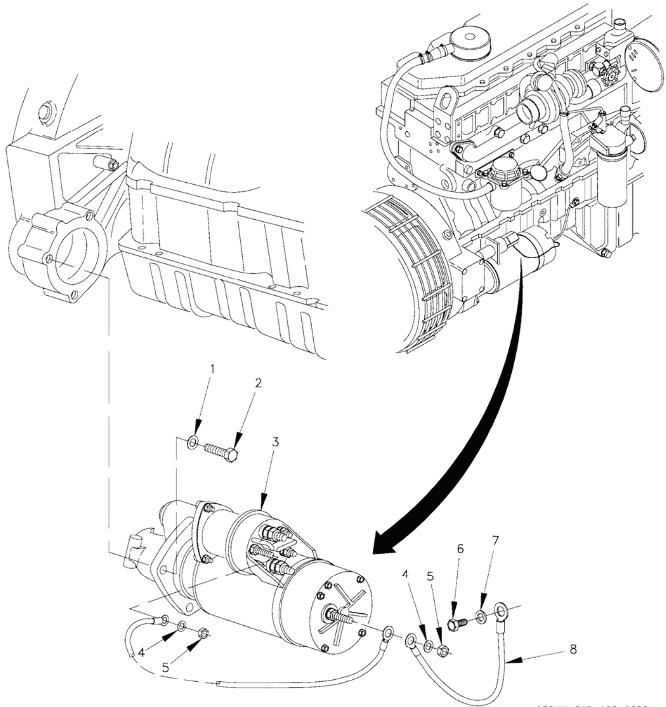
Figure 23. Starting Motor Group.
