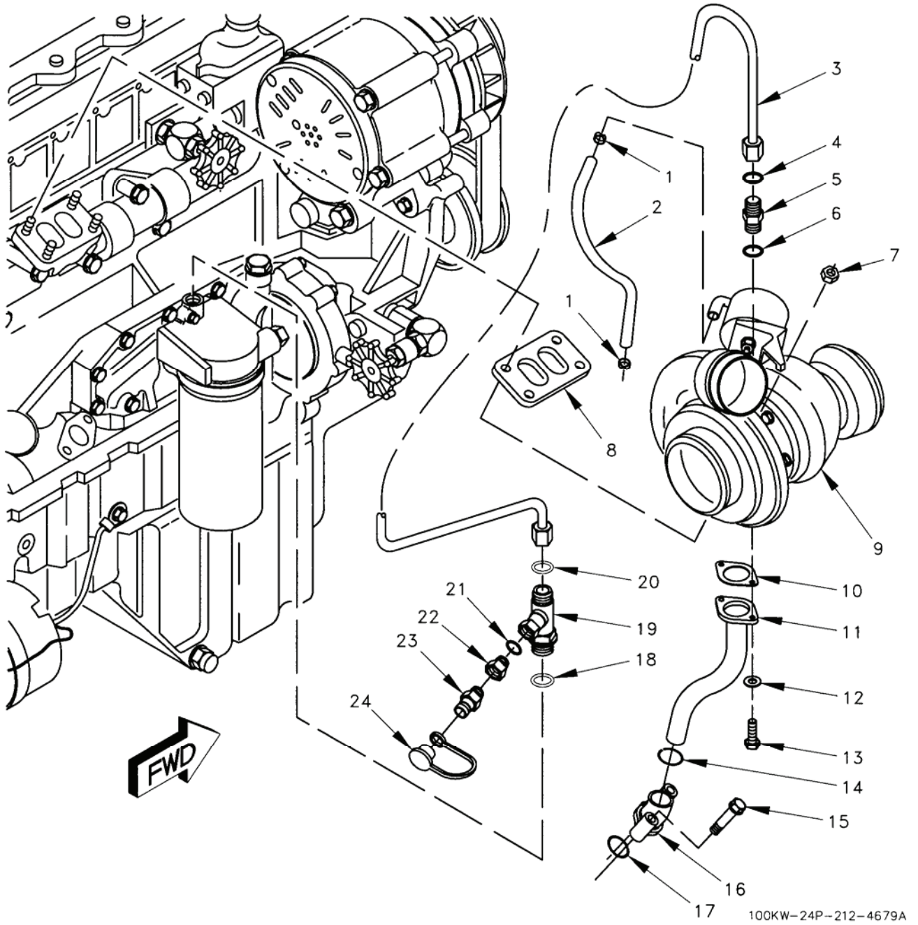
Figure 26. Turbocharger Group.
