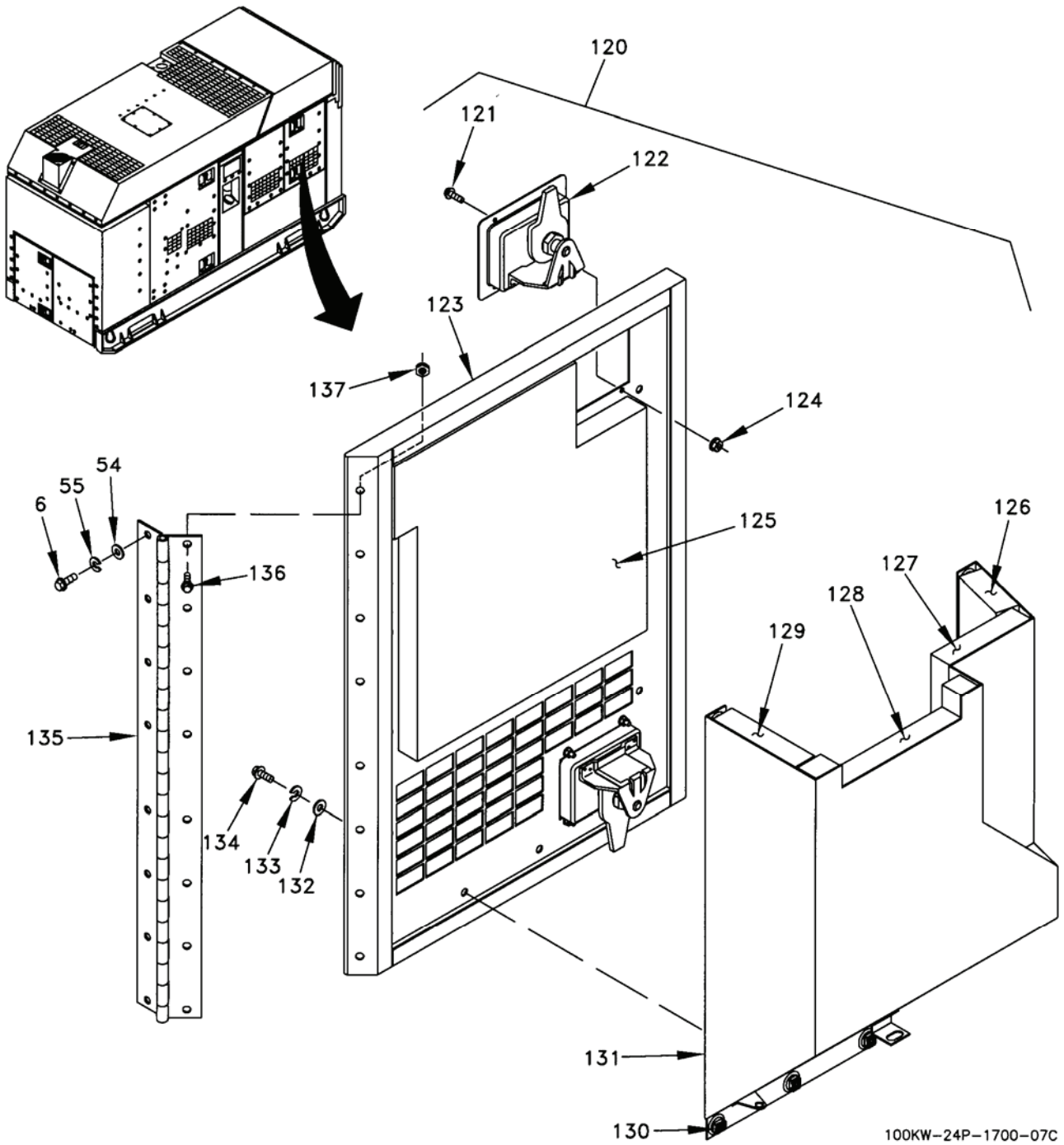
Figure 3. Housing Installation (Sheet 7 of 25).
