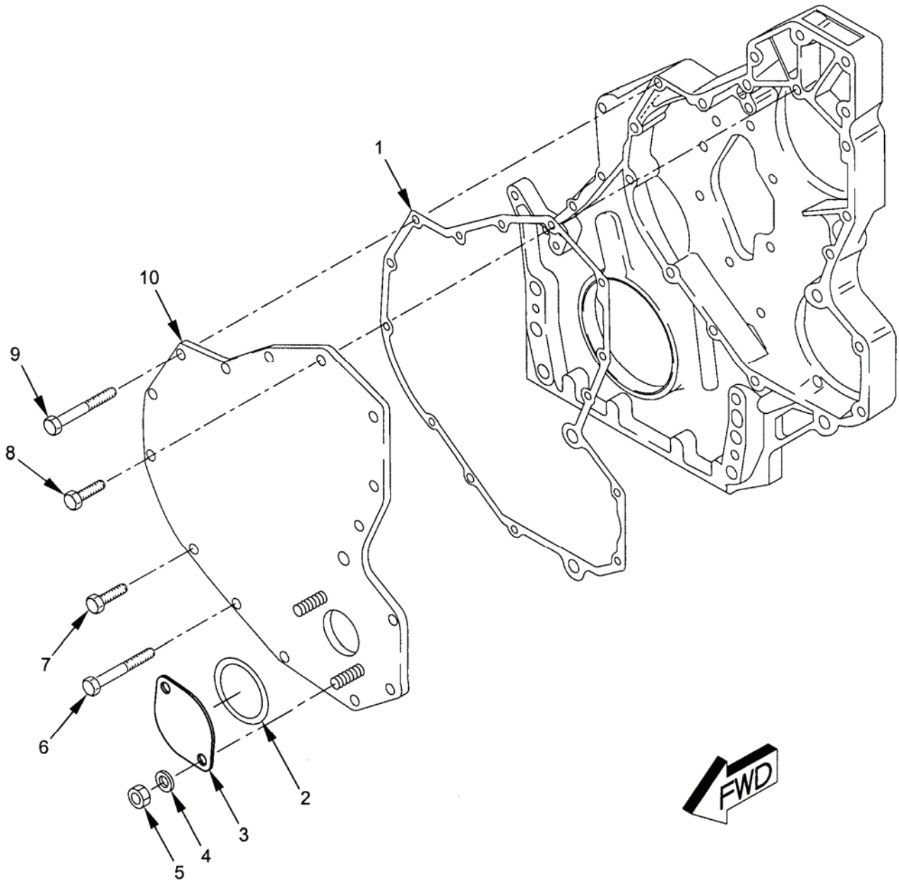
Figure 46. Front Cover Group.
