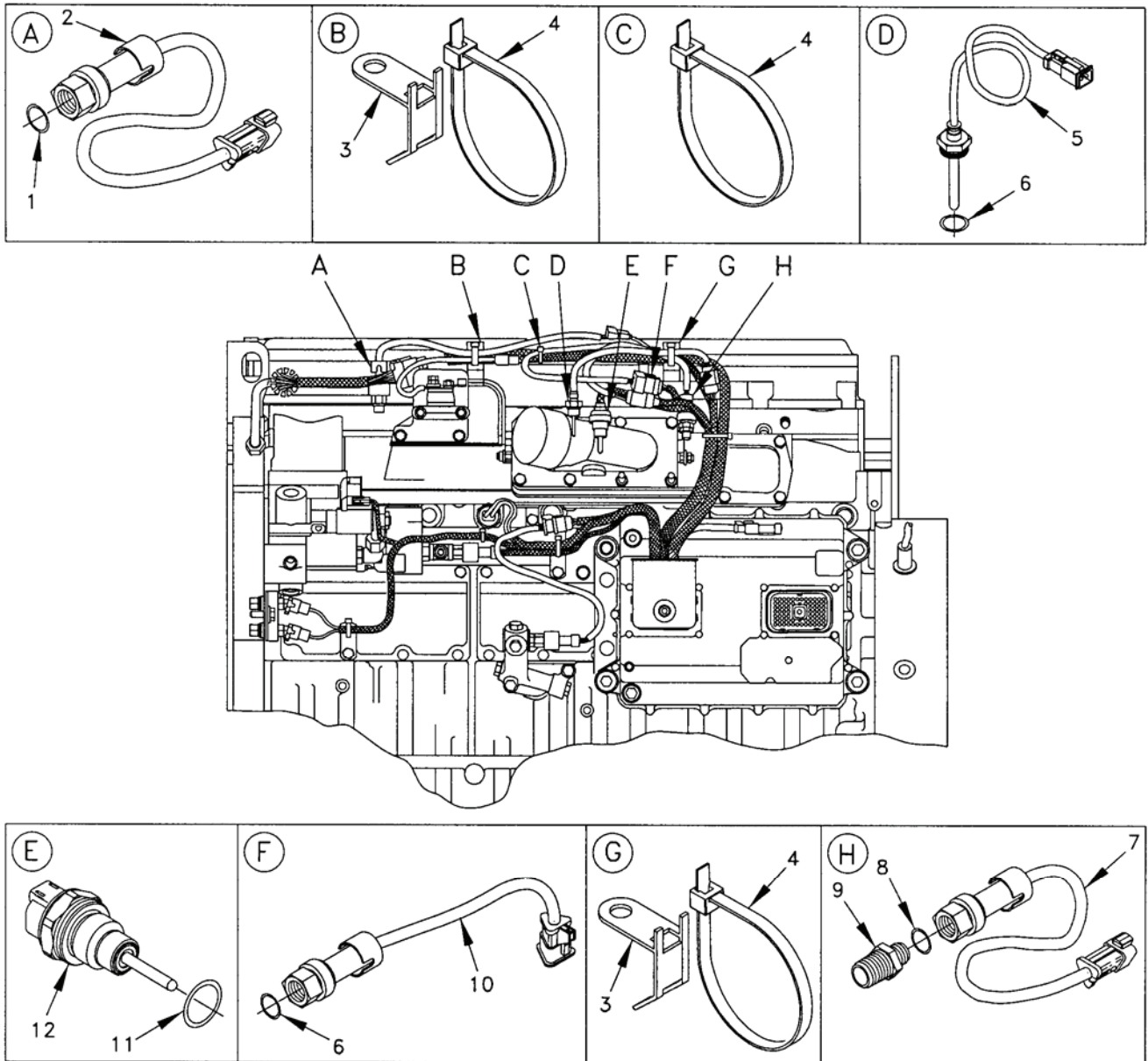
Figure 24. Sensor and Wiring Group (Sheet 1 of 4).
