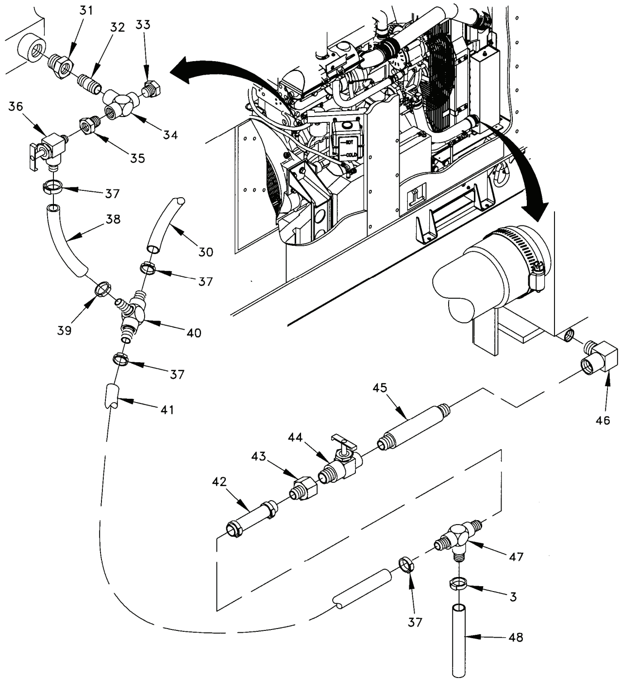
Figure 13. Cooling System Installation (Sheet 3 of 6).
