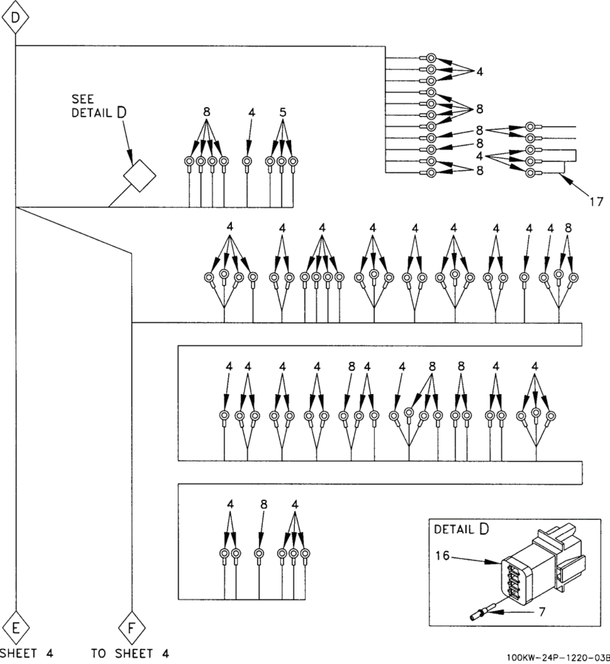
Figure 5. Control Box Harness Assembly (Sheet 3 of 5).
