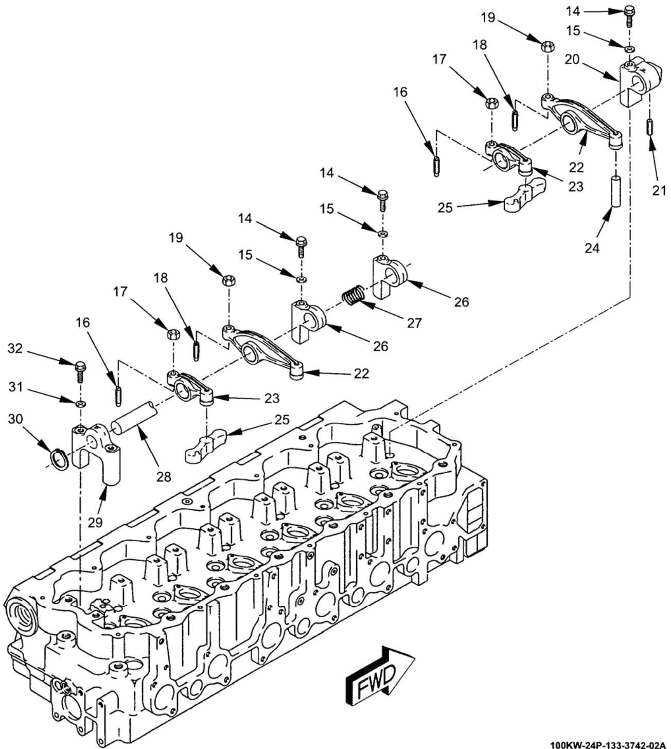
Figure 38. Cylinder Head Group (Sheet 2 of 3).
