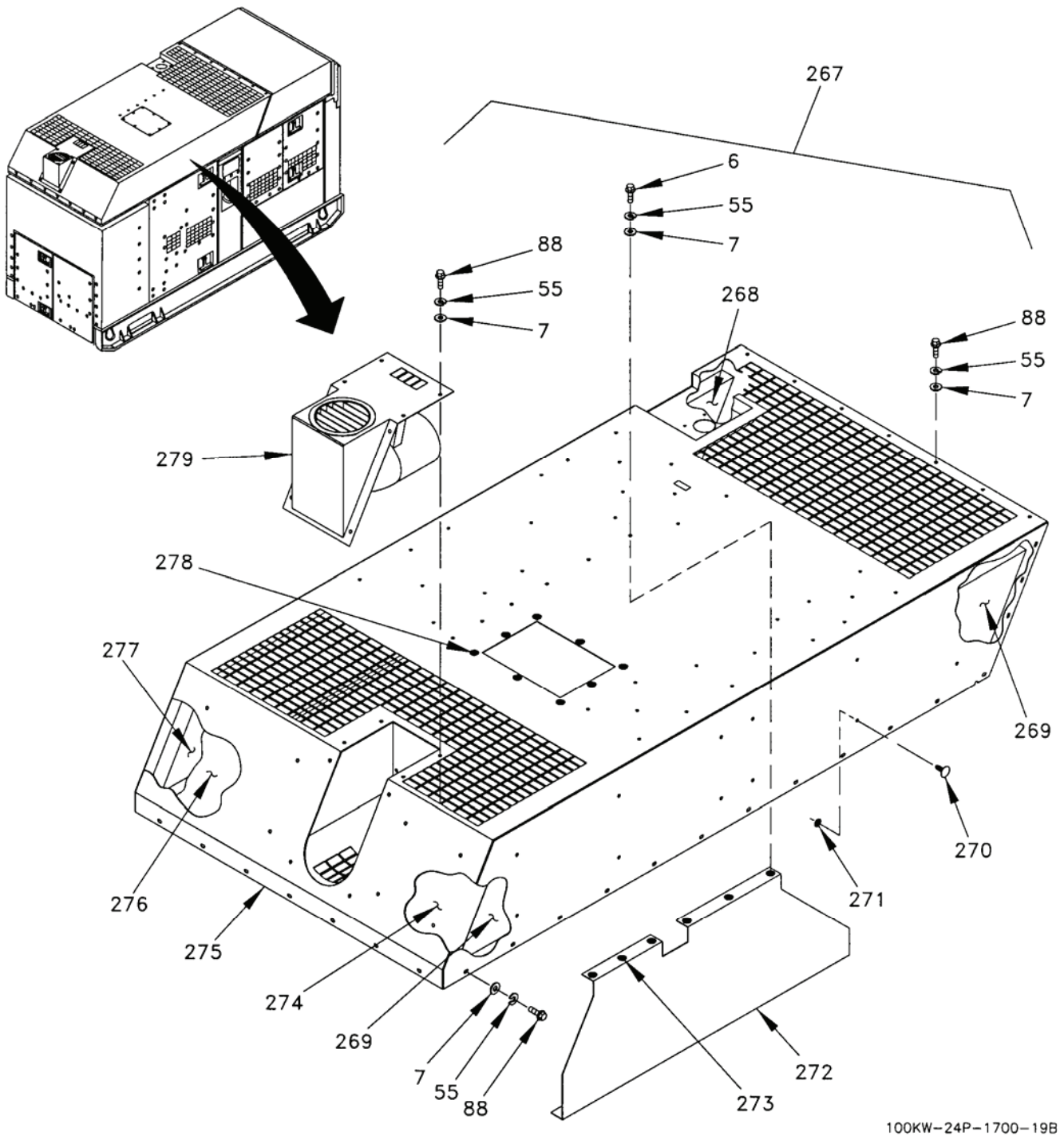
Figure 3. Housing Installation (Sheet 19 of 25).
