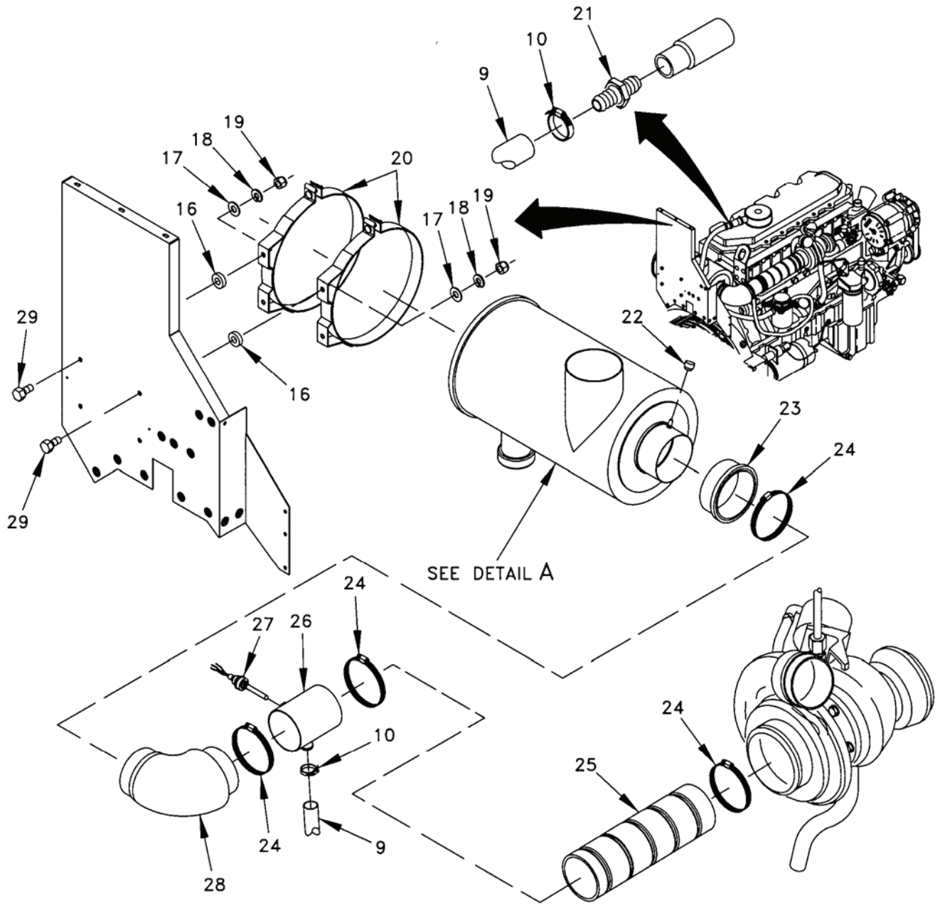
Figure 15. Air Cleaner Installation (Sheet 2 of 3).
