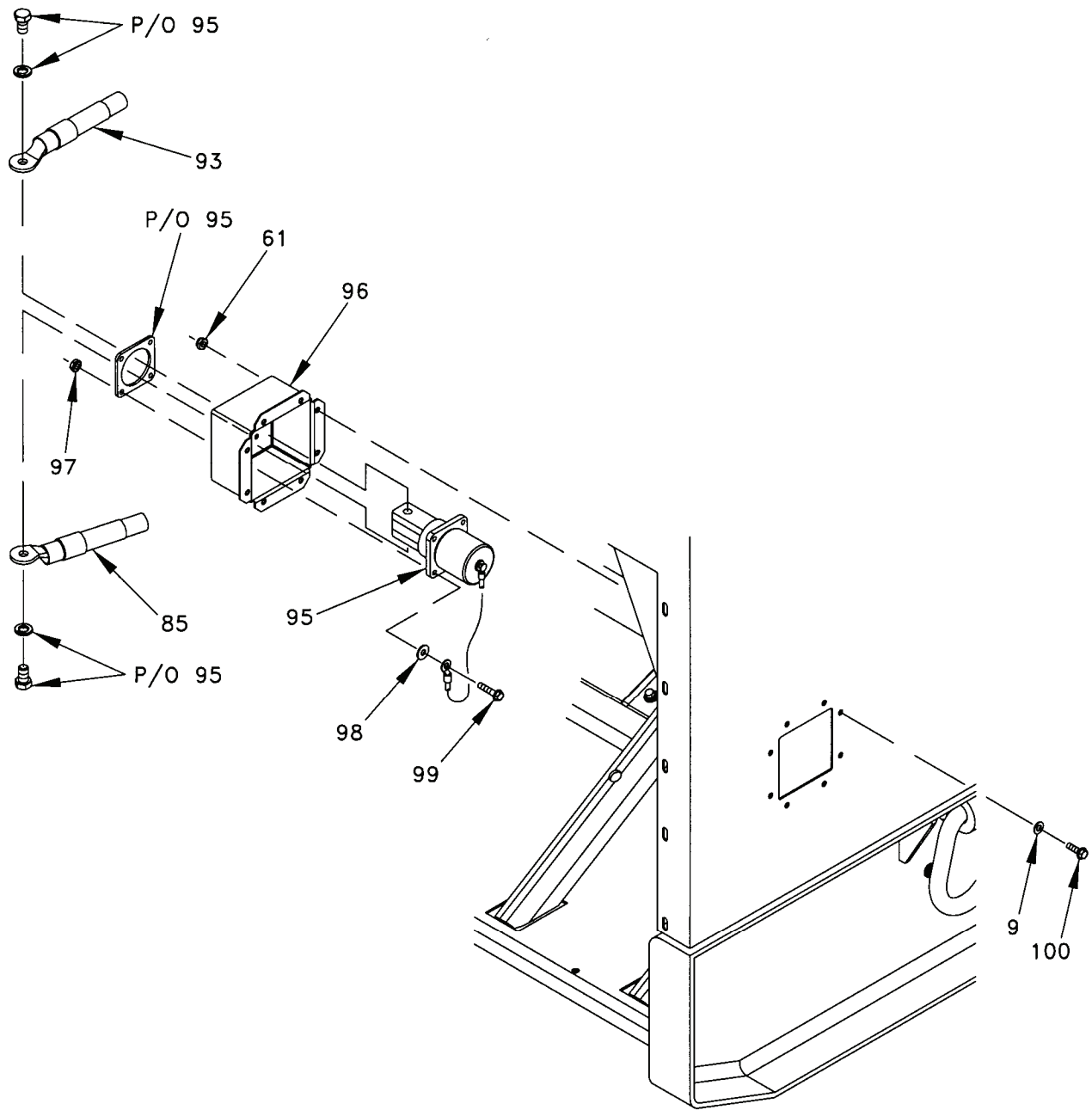
Figure 7. Electrical Components Installation (Sheet 7 of 8).
