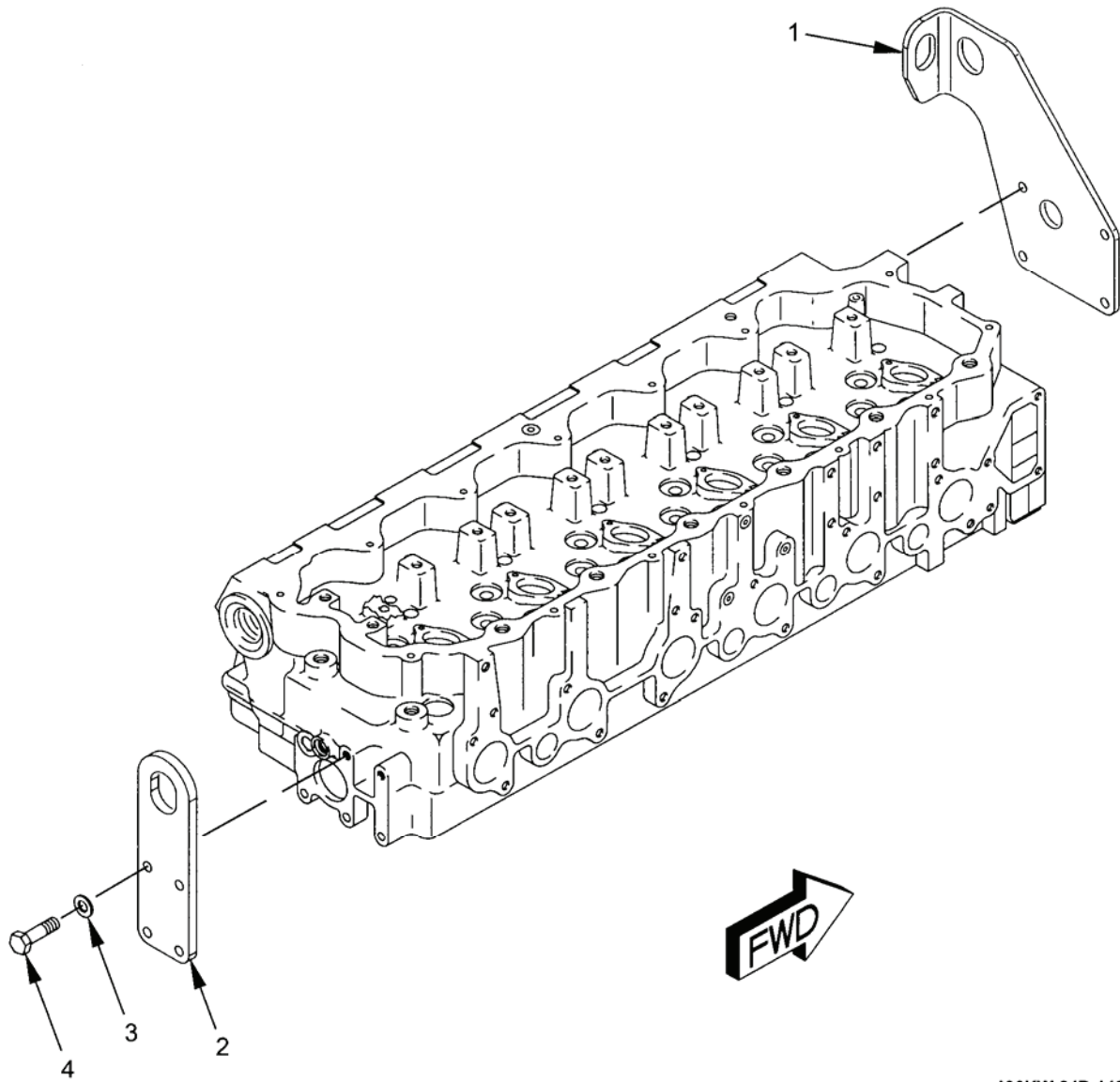
Figure 22. Lifting Group.
