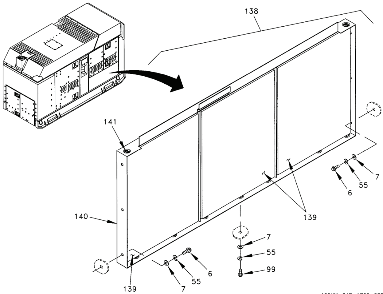
Figure 3. Housing Installation (Sheet 8 of 25).
