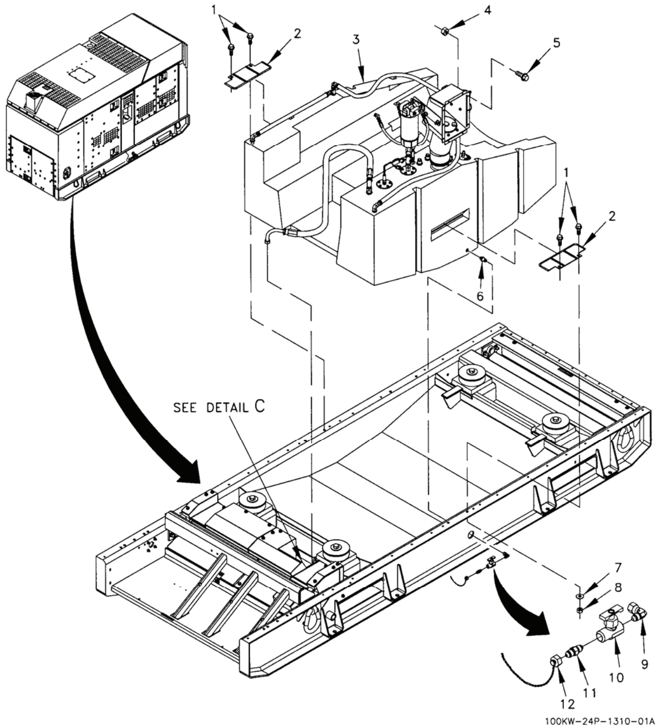
Figure 12. Fuel System Installation (Sheet 1 of 4).
