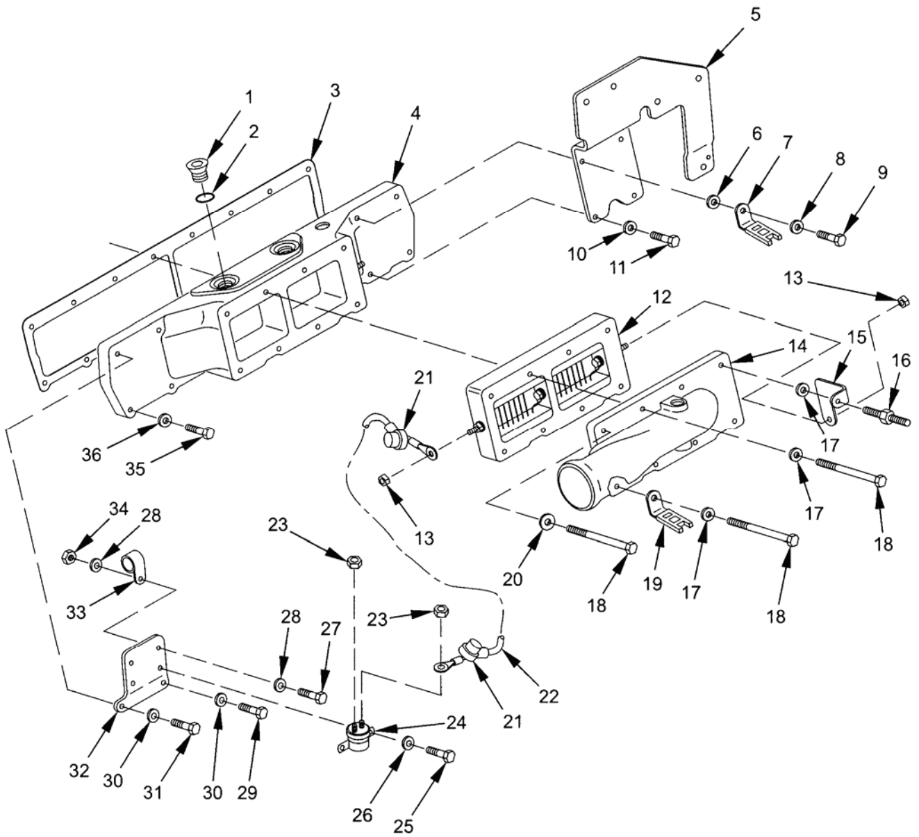
Figure 28. Heater and Air Inlet Group.
