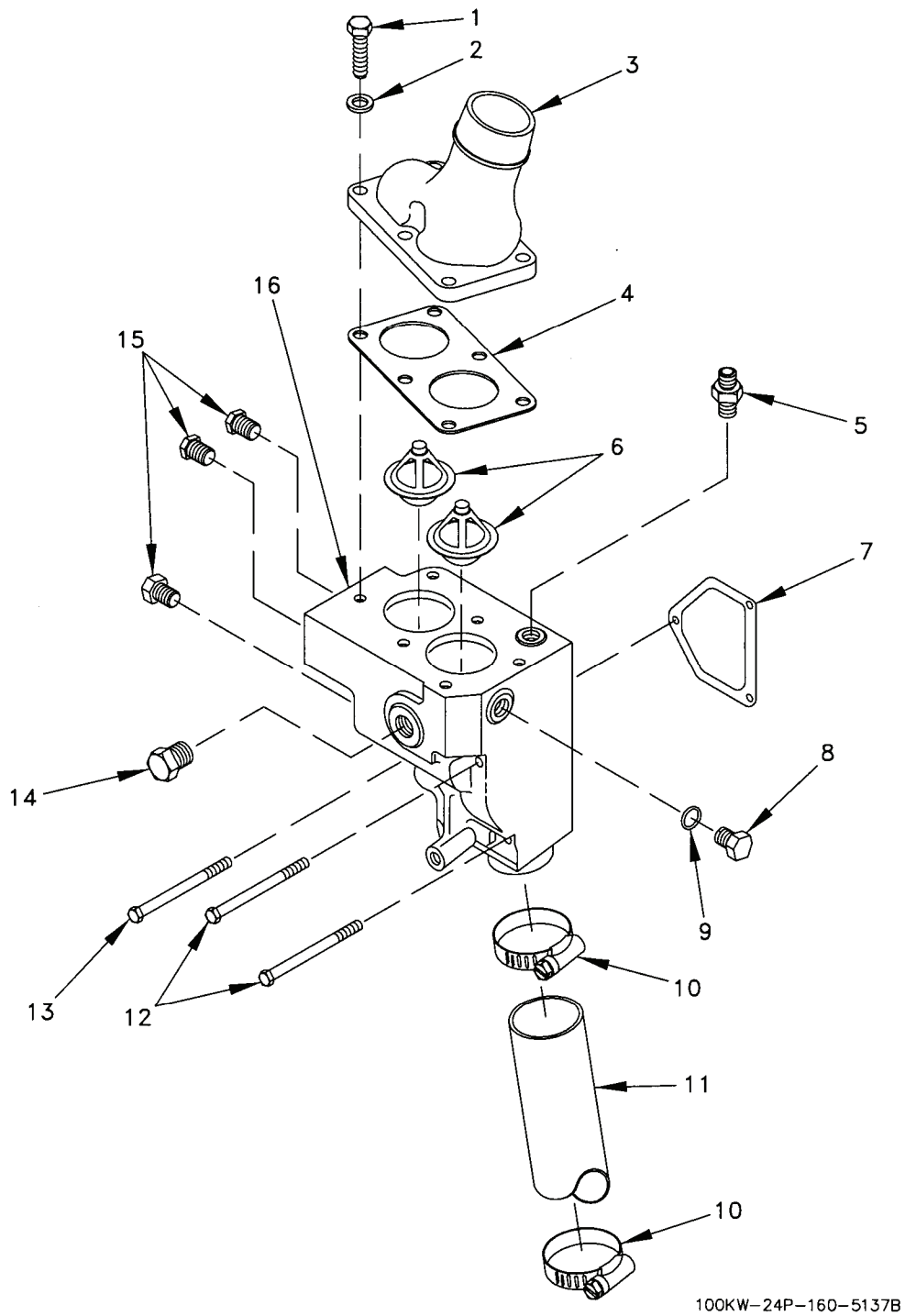
Figure 21. Water Line Group.
