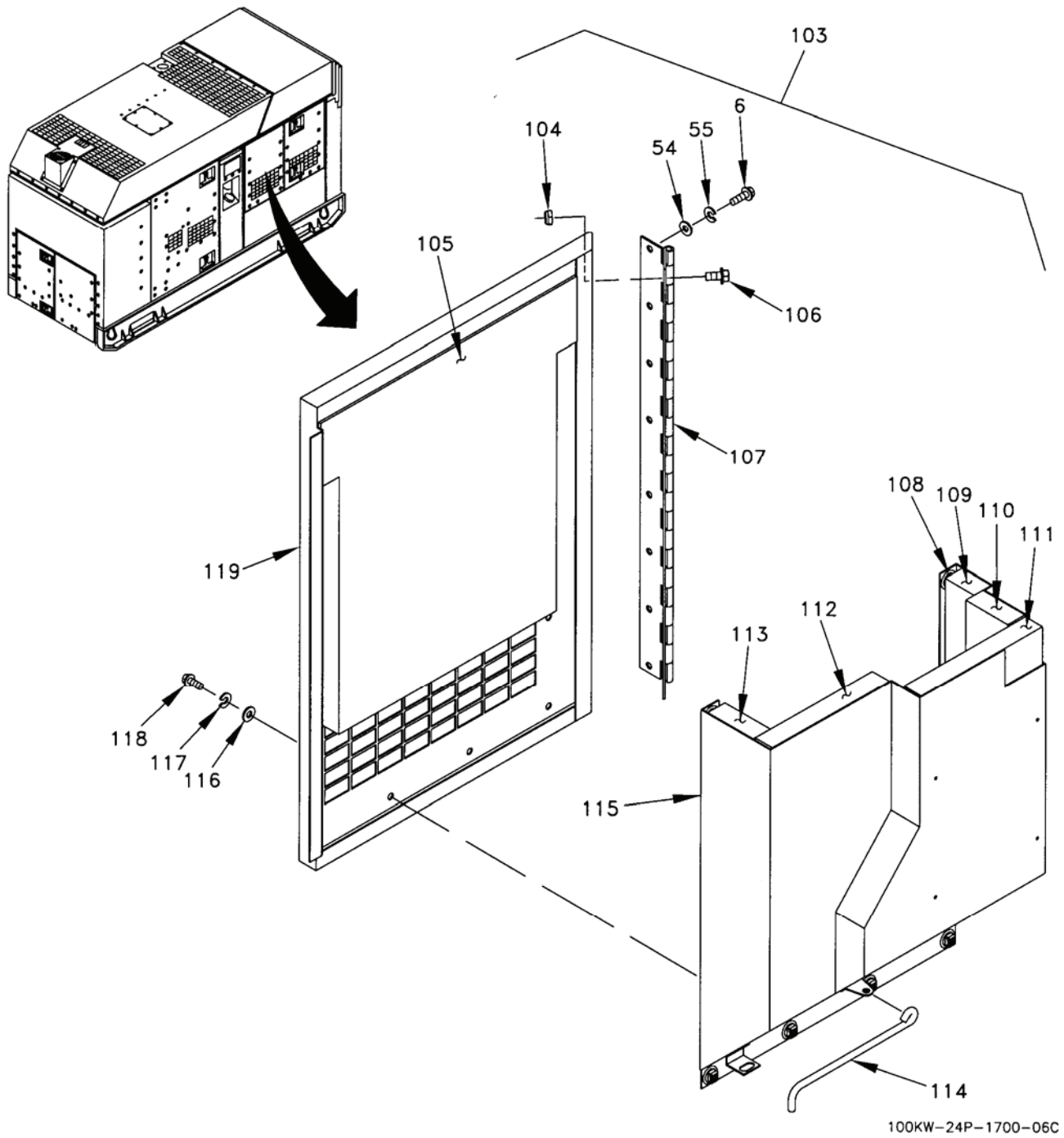
Figure 3. Housing Installation (Sheet 6 of 25).
