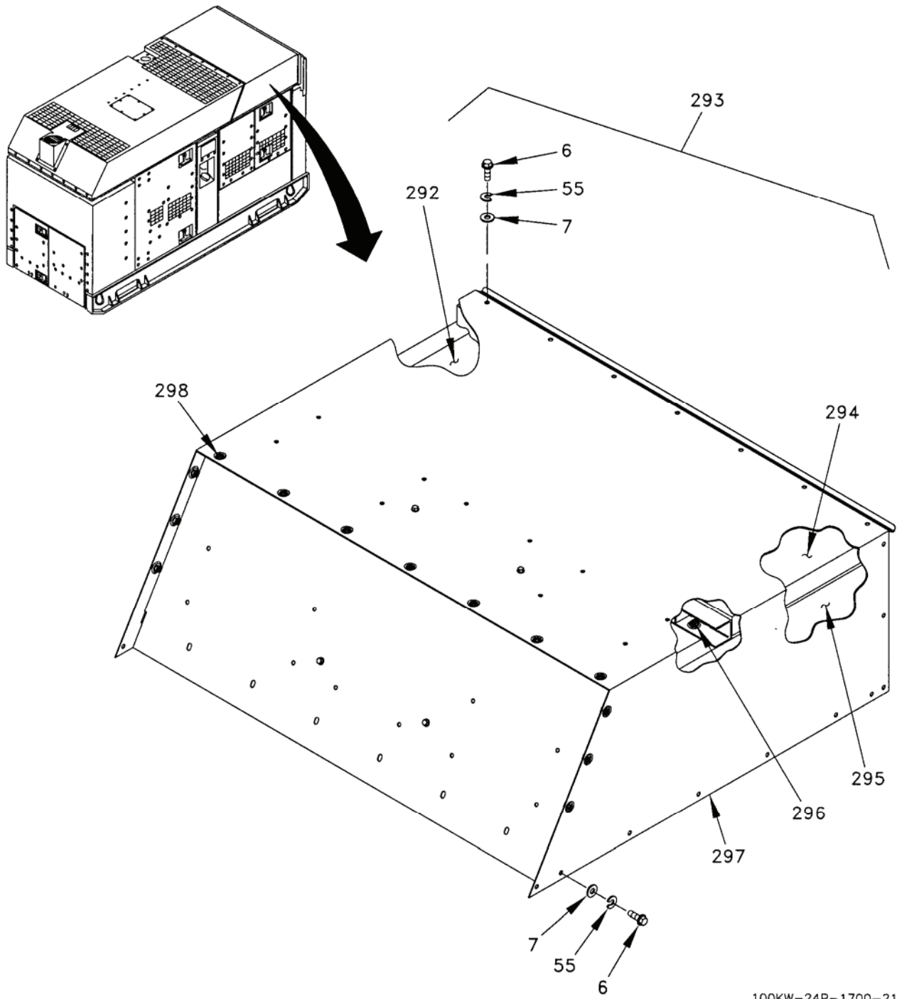
Figure 3. Housing Installation (Sheet 21 of 25).
