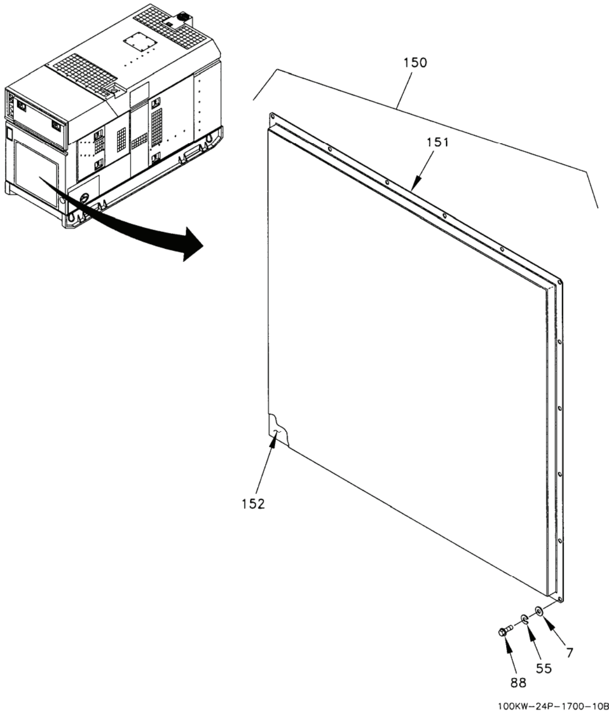
Figure 3. Housing Installation (Sheet 10 of 25).
