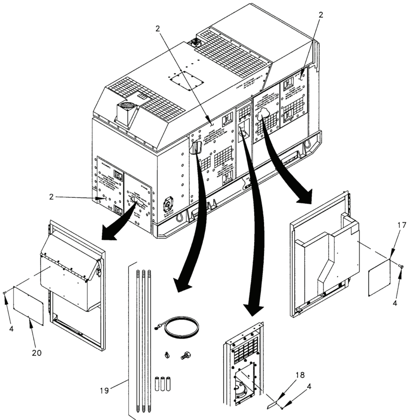
Figure 1. Generator Set, Tactical Quiet, 100 kW, 50/60 Hz (Sheet 2 of 3).
