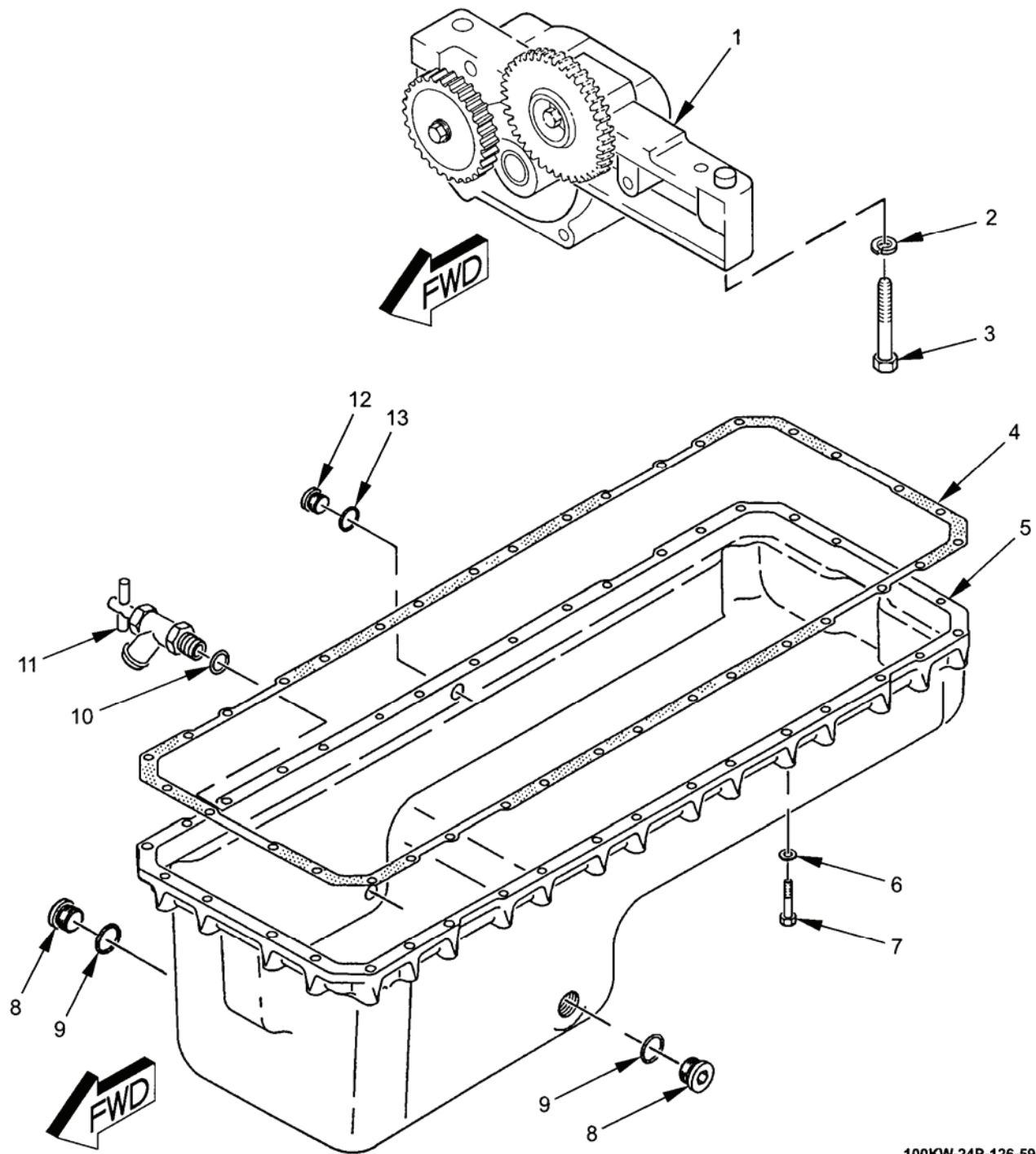
Figure 29. Oil Pan Group.
