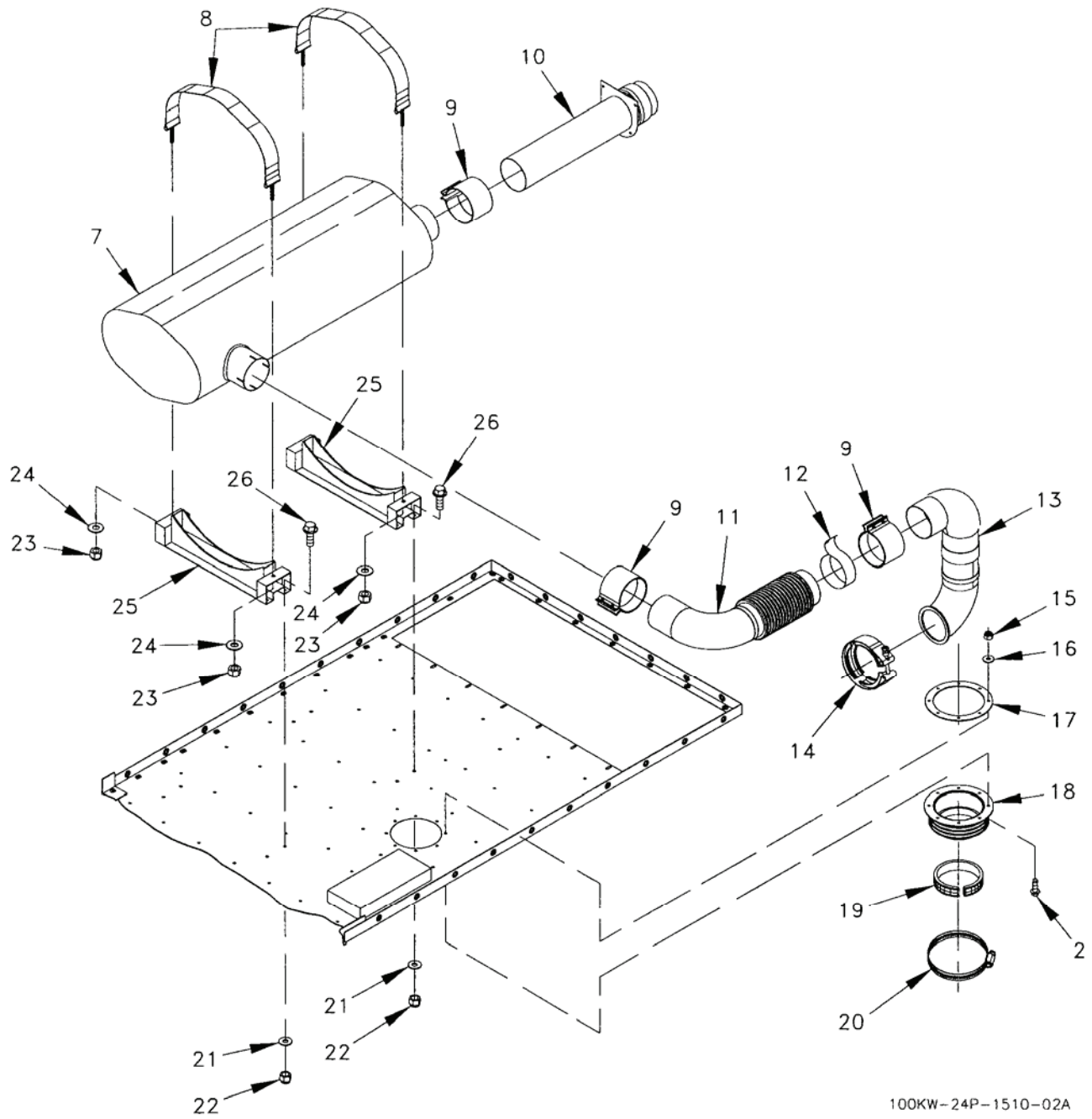
Figure 14. Exhaust System Installation (Sheet 2 of 2).
