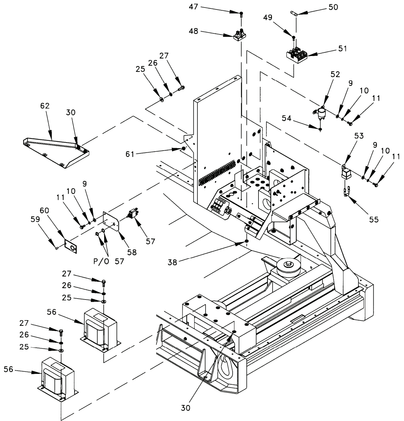
Figure 7. Electrical Components Installation (Sheet 3 of 8).
