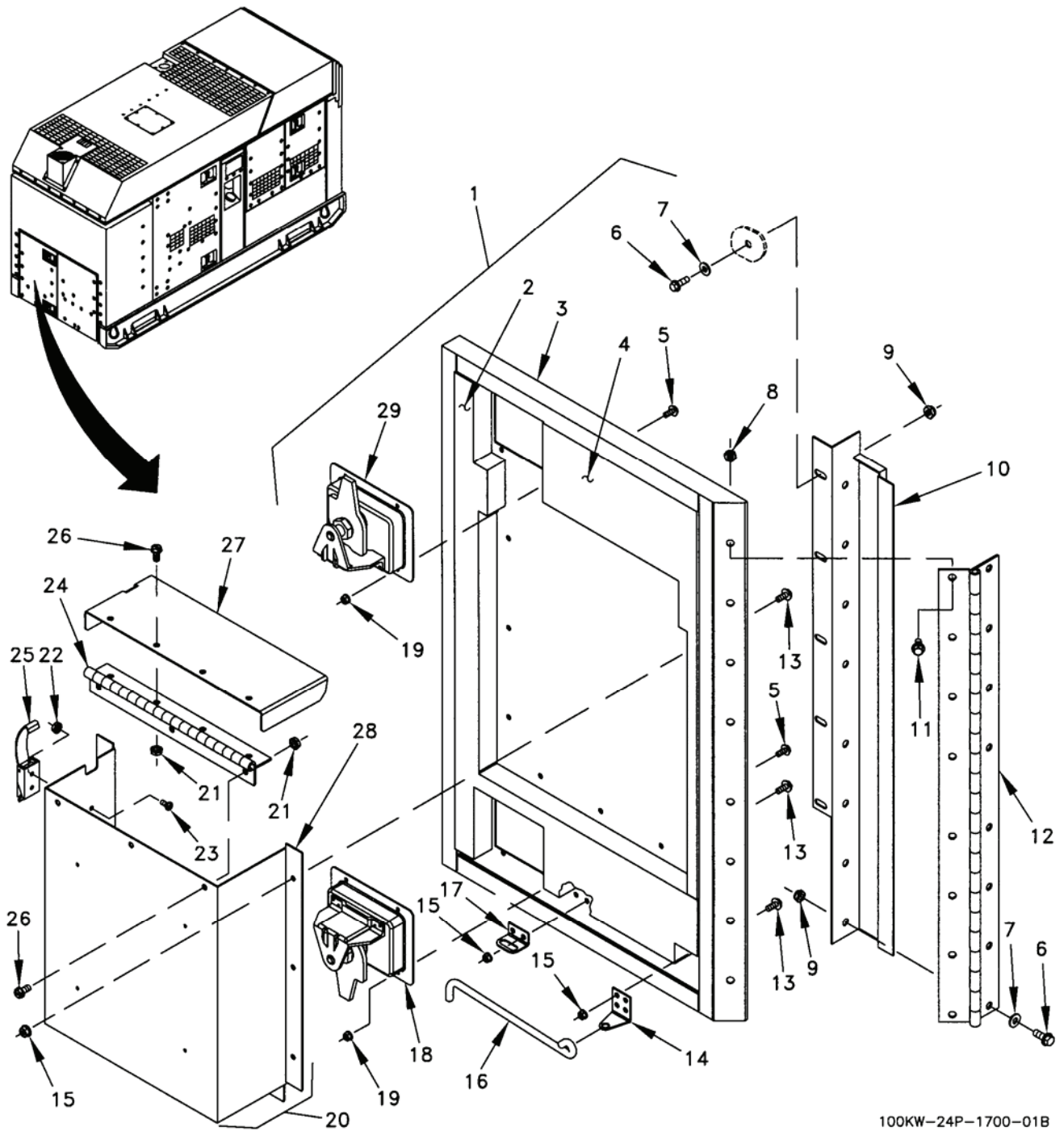
Figure 3. Housing Installation (Sheet 1 of 25).
