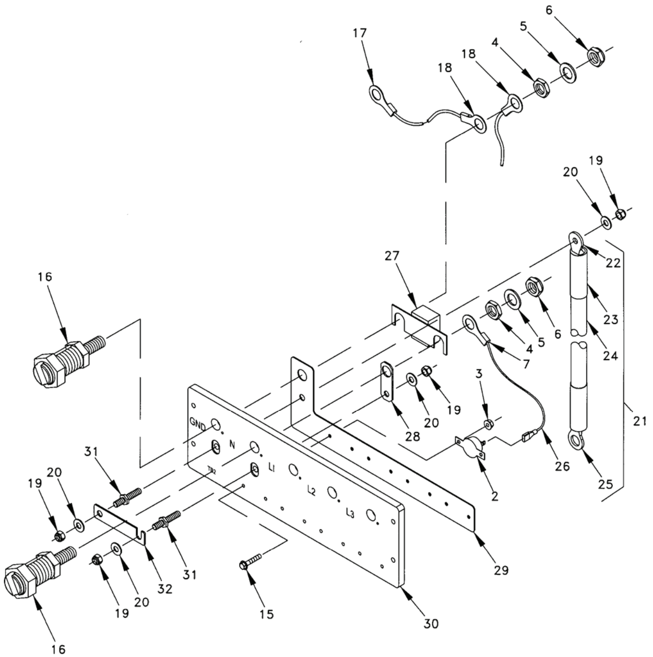
Figure 11. Load Terminal Board Assembly (Sheet 2 of 2).
