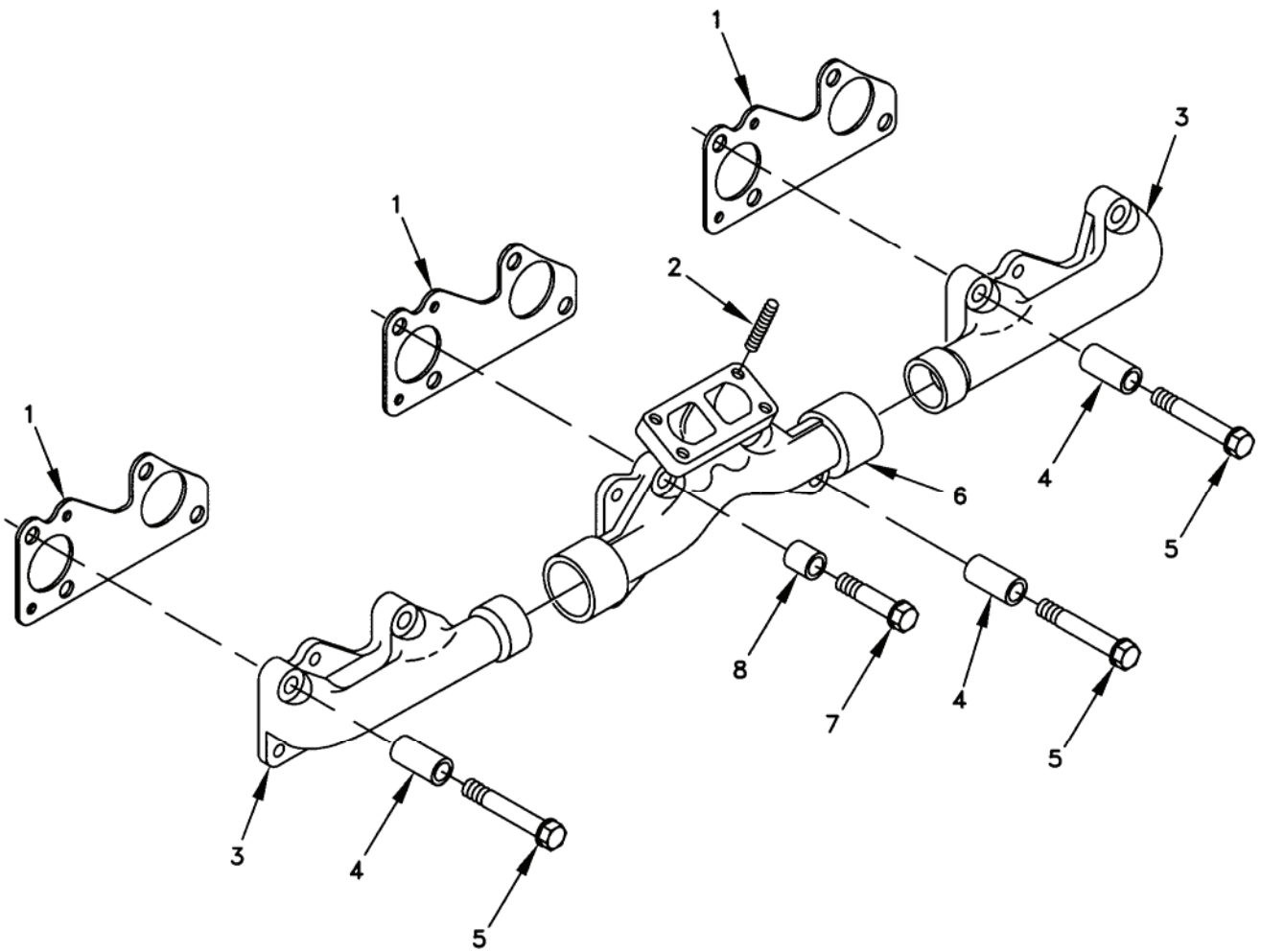
Figure 27. Exhaust Manifold Group.
