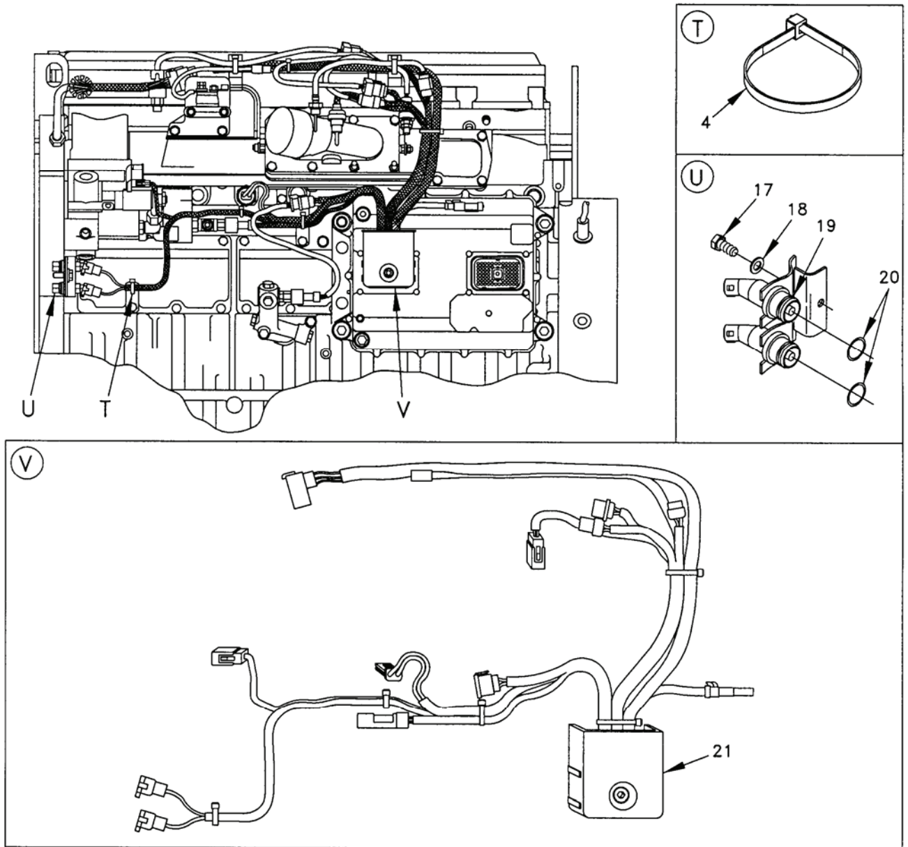
Figure 24. Sensor and Wiring Group (Sheet 3 of 4).
