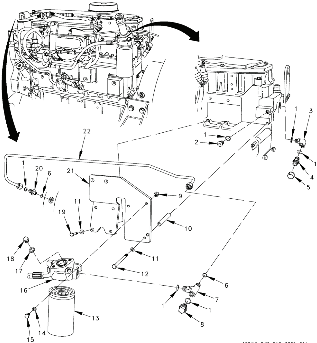
Figure 37. Fuel Filter and Line Group (Sheet 1 of 2).
