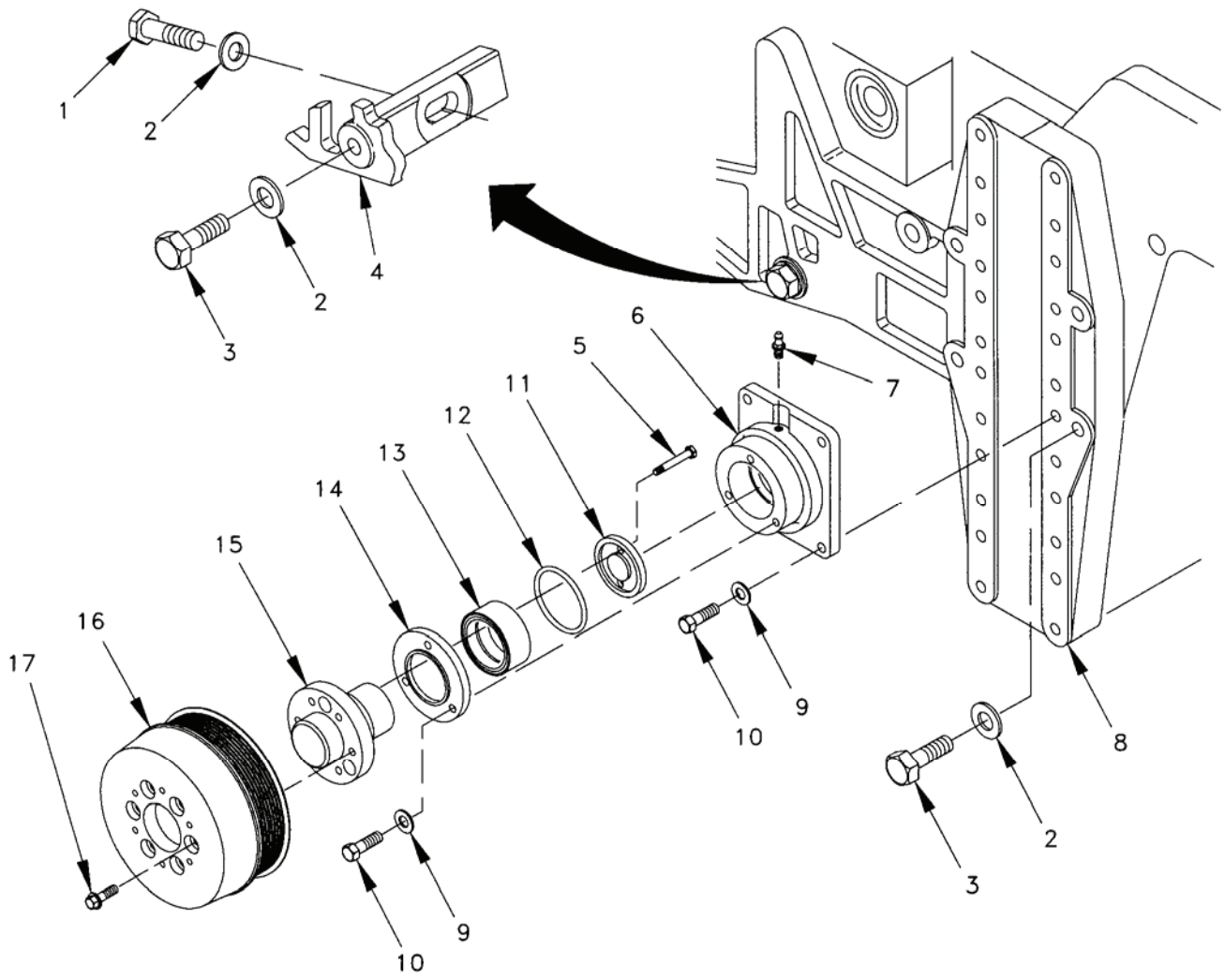
Figure 19. Engine Pulley Group.
