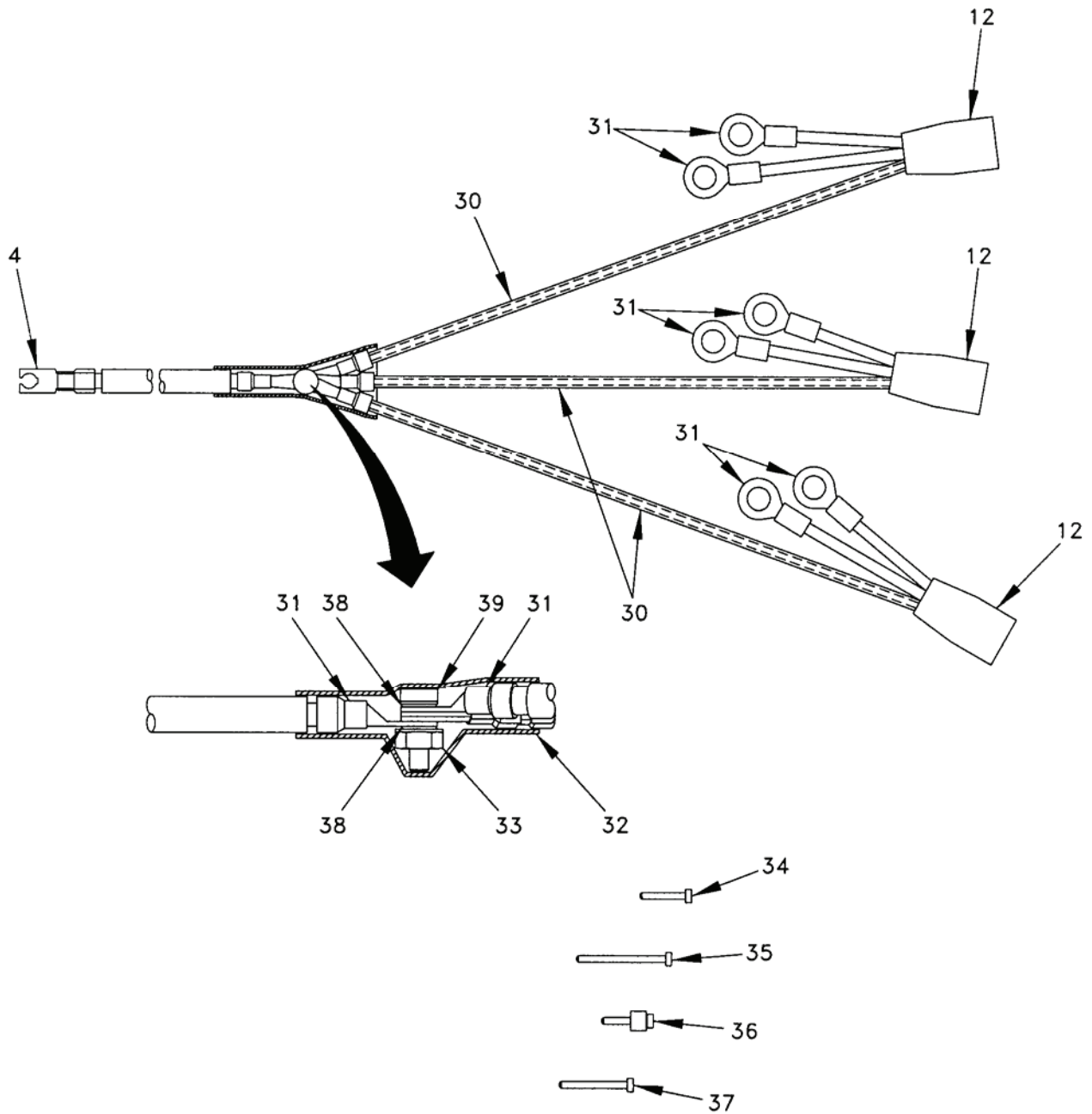
Figure 5. Control Box Harness Assembly (Sheet 5 of 5).
