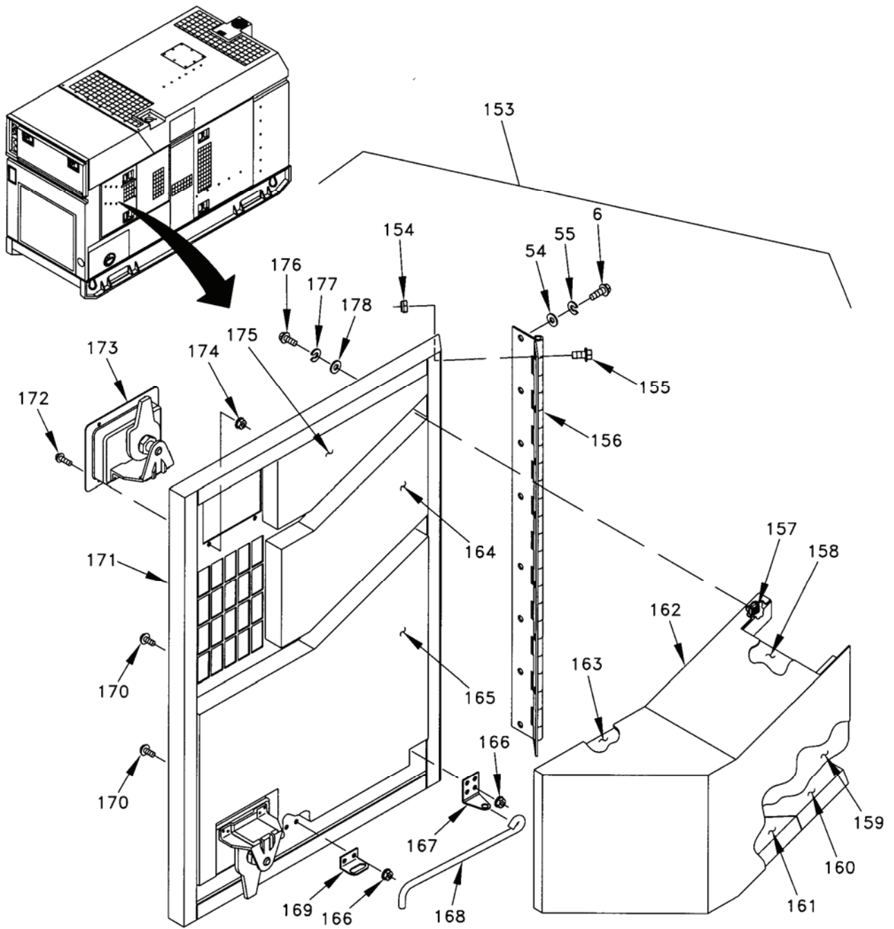
Figure 3. Housing Installation (Sheet 11 of 25).
