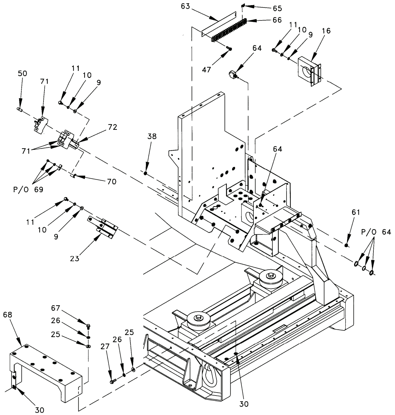
Figure 7. Electrical Components Installation (Sheet 4 of 8).
