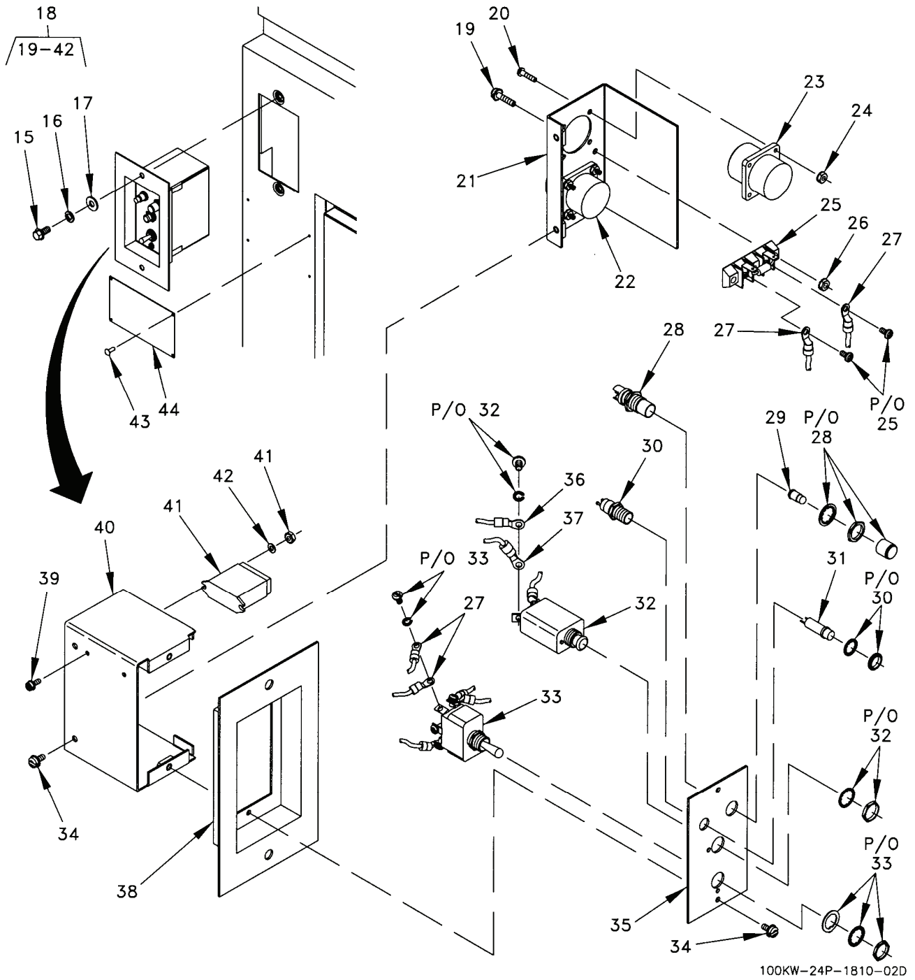
Figure 53. Winterization Kit Installation (Sheet 2 of 5).
