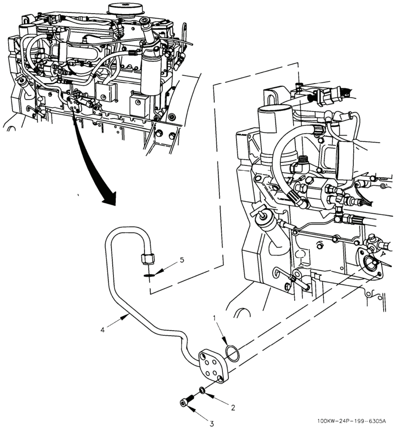
Figure 33. Oil Line Group.
