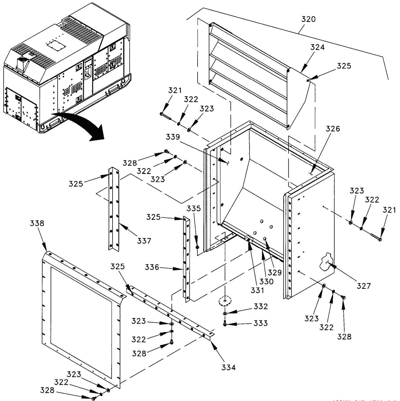
Figure 3. Housing Installation (Sheet 24 of 25).
