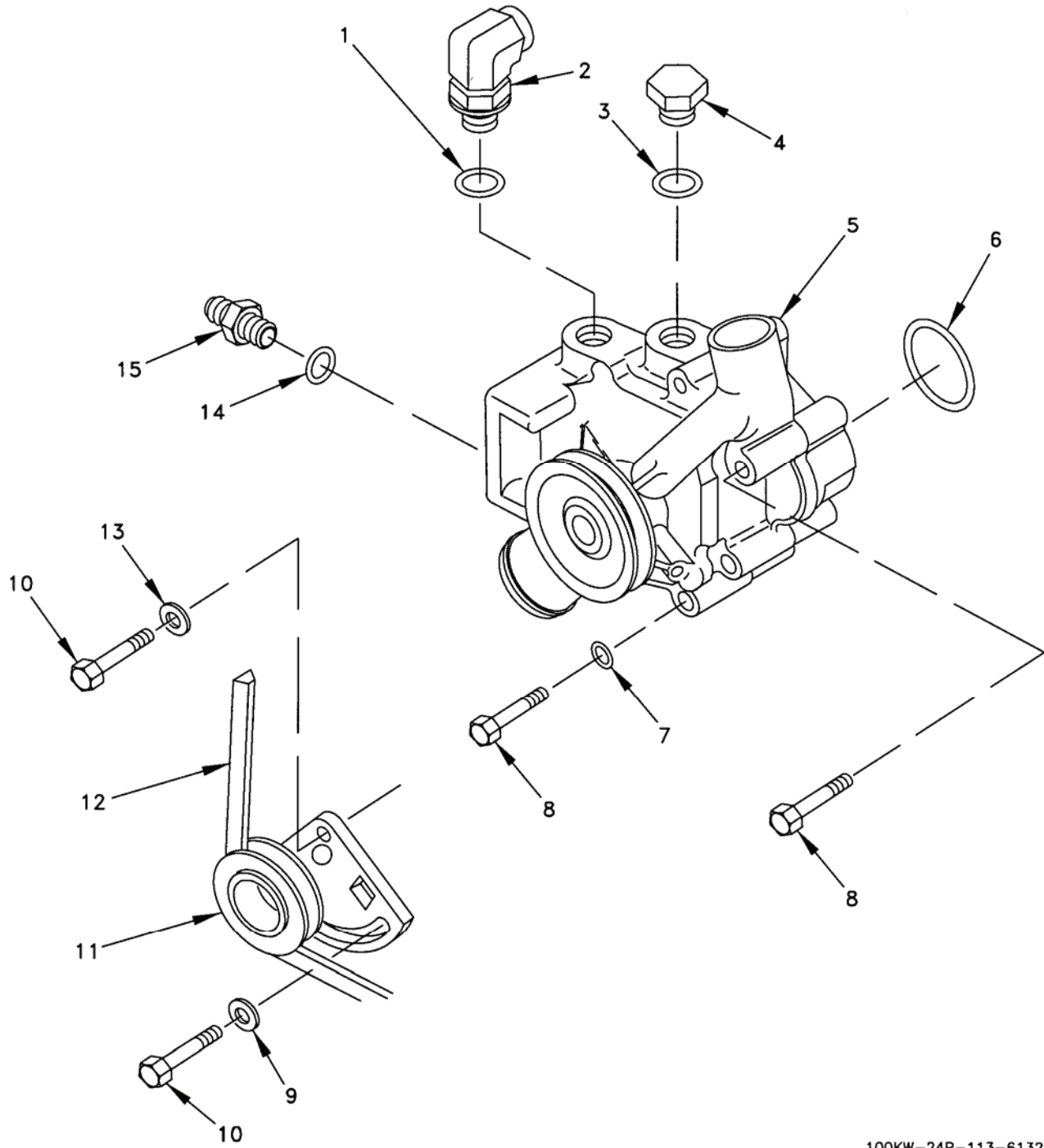
Figure 20. Water Pump Group.
