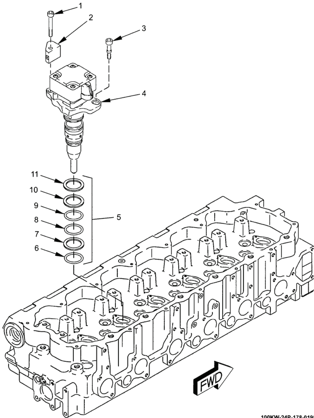
Figure 39. Fuel Injection Pump Group.
