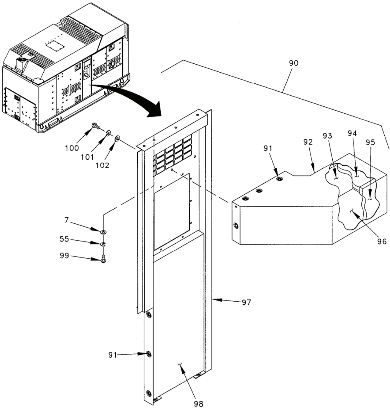
Figure 3. Housing Installation (Sheet 5 of 25).
