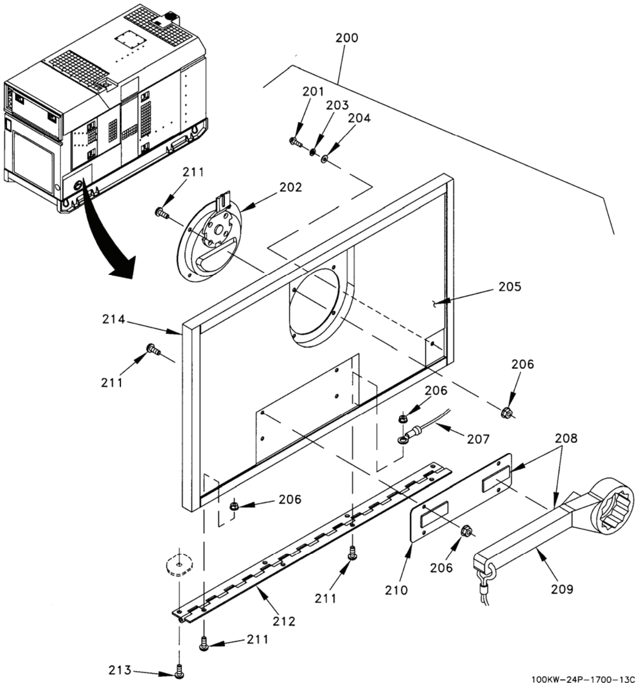
Figure 3. Housing Installation (Sheet 13 of 25).
