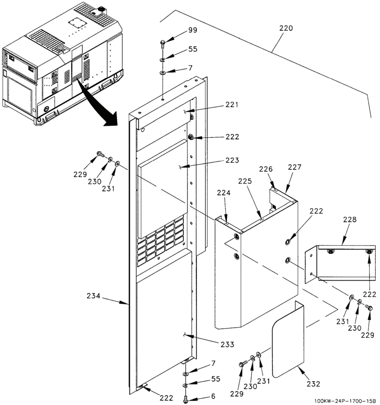
Figure 3. Housing Installation (Sheet 15 of 25).
