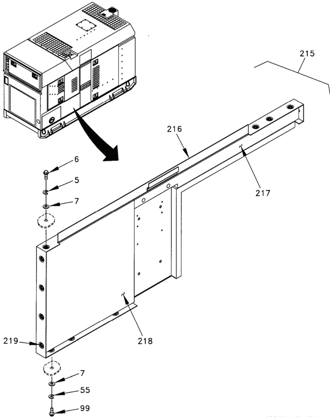
Figure 3. Housing Installation (Sheet 14 of 25).
