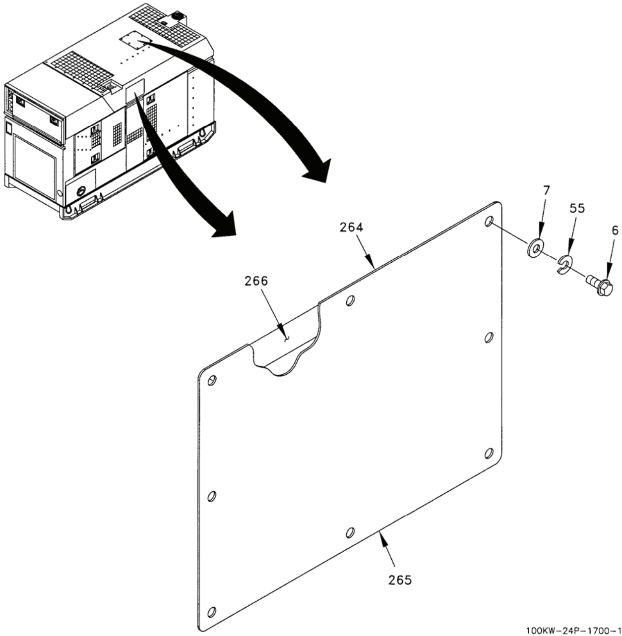
Figure 3. Housing Installation (Sheet 18 of 25).
