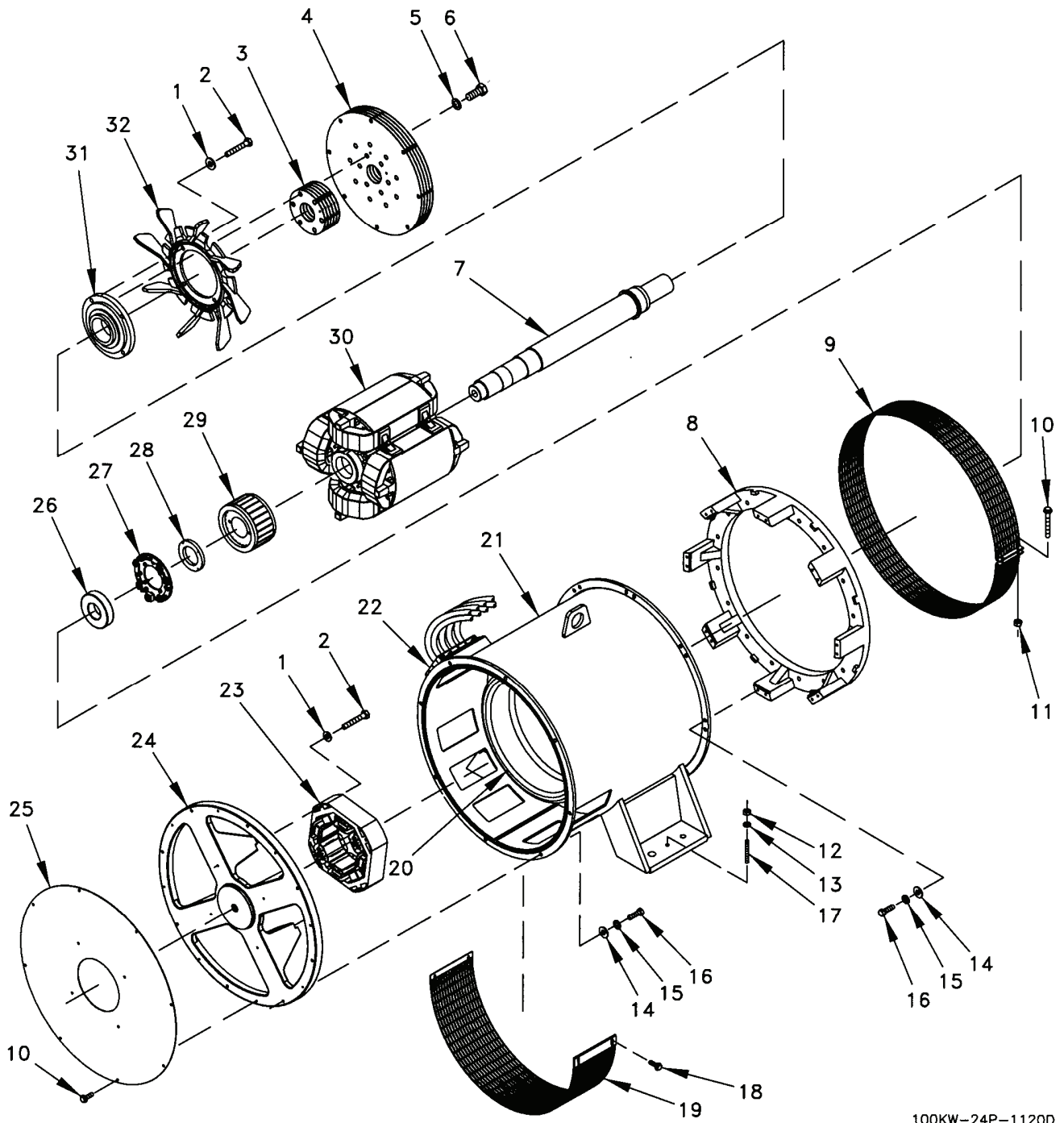
Figure 17. Generator.
