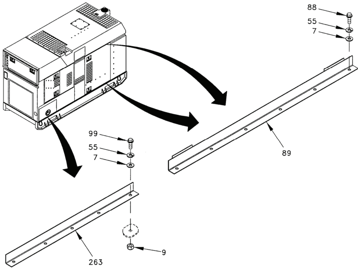
Figure 3. Housing Installation (Sheet 17 of 25).
