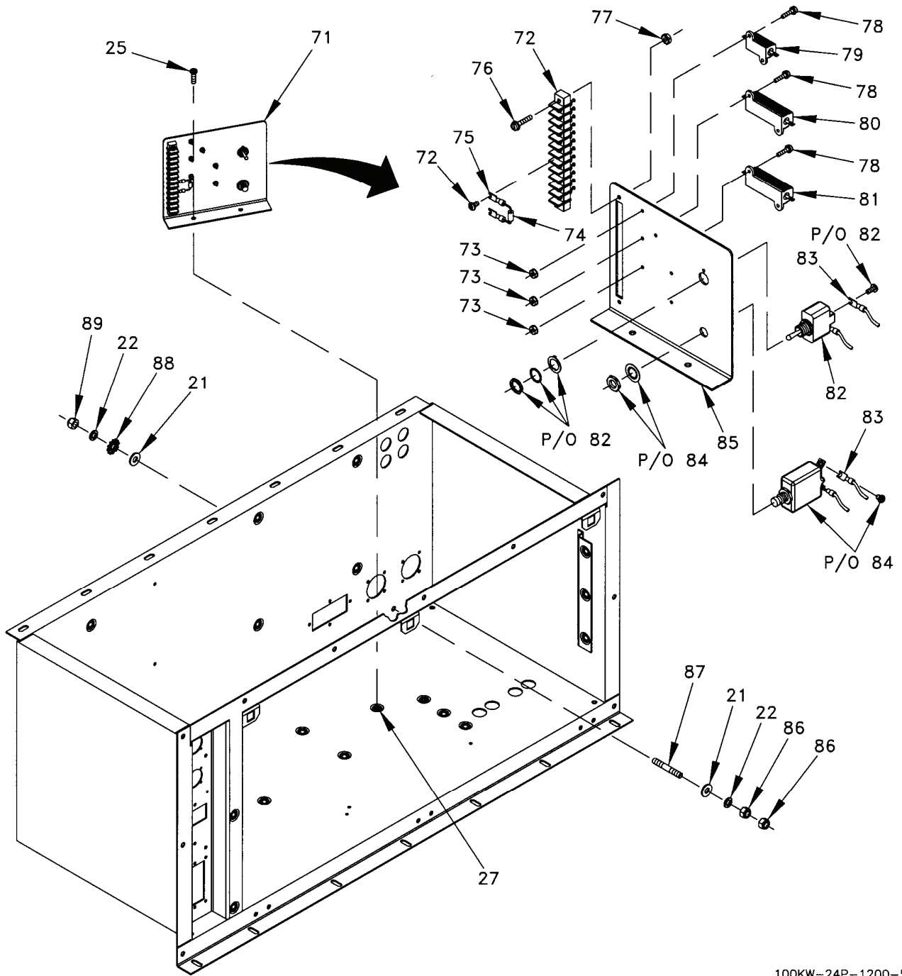
Figure 4. Control Box Assembly (Sheet 5 of 5).
