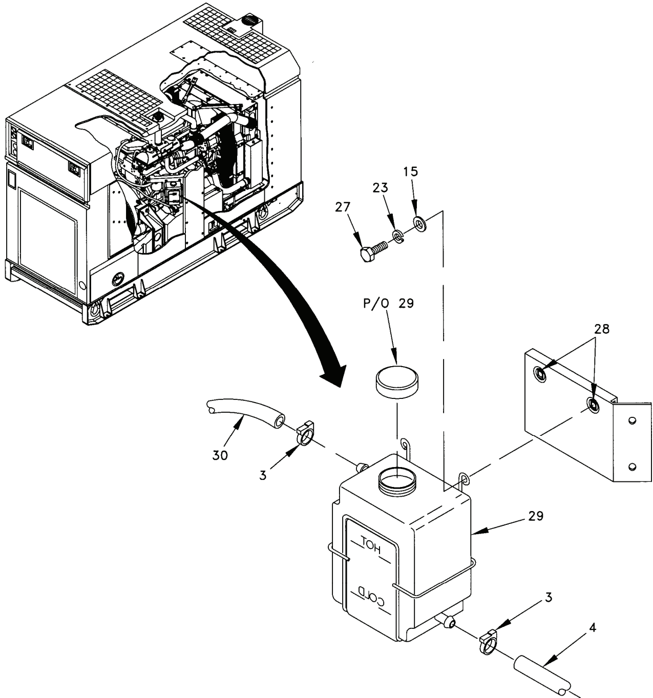
Figure 13. Cooling System Installation (Sheet 2 of 6).
