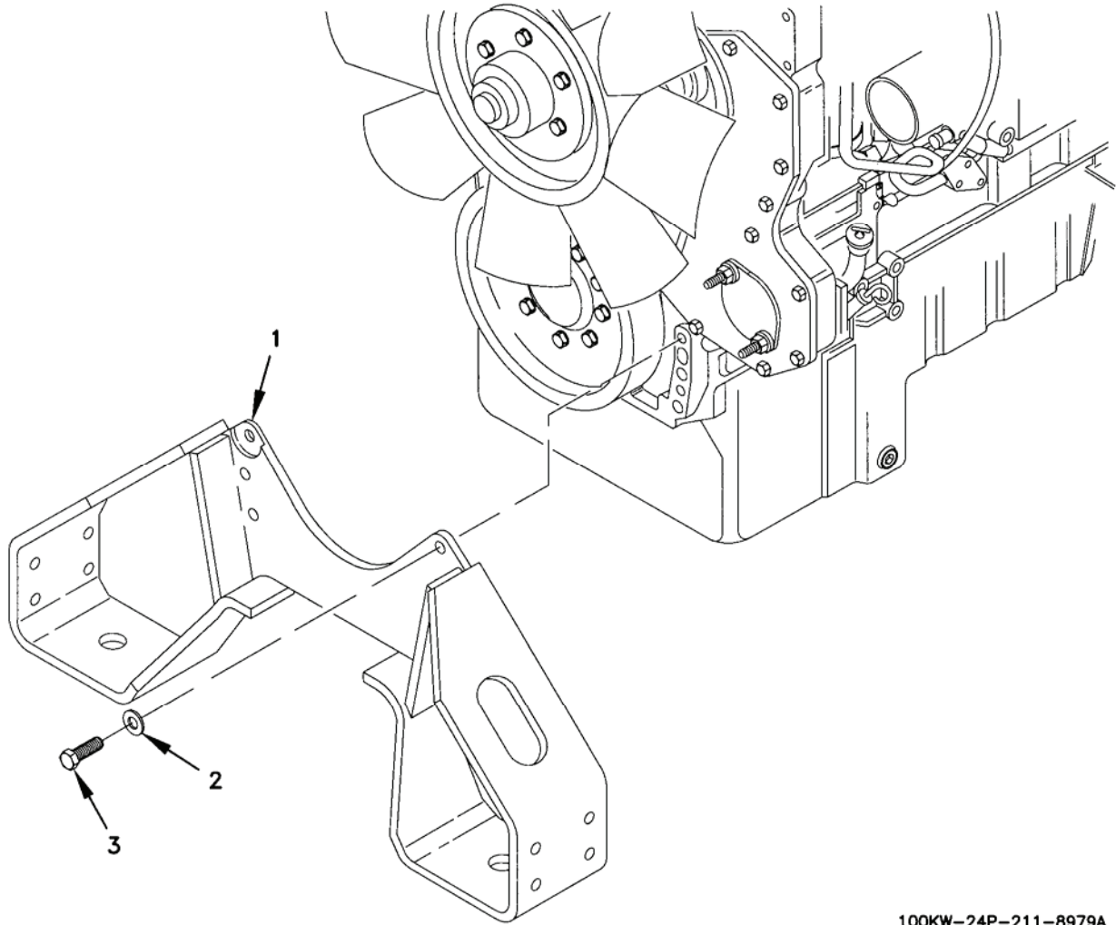
Figure 49. Engine Support Group.
