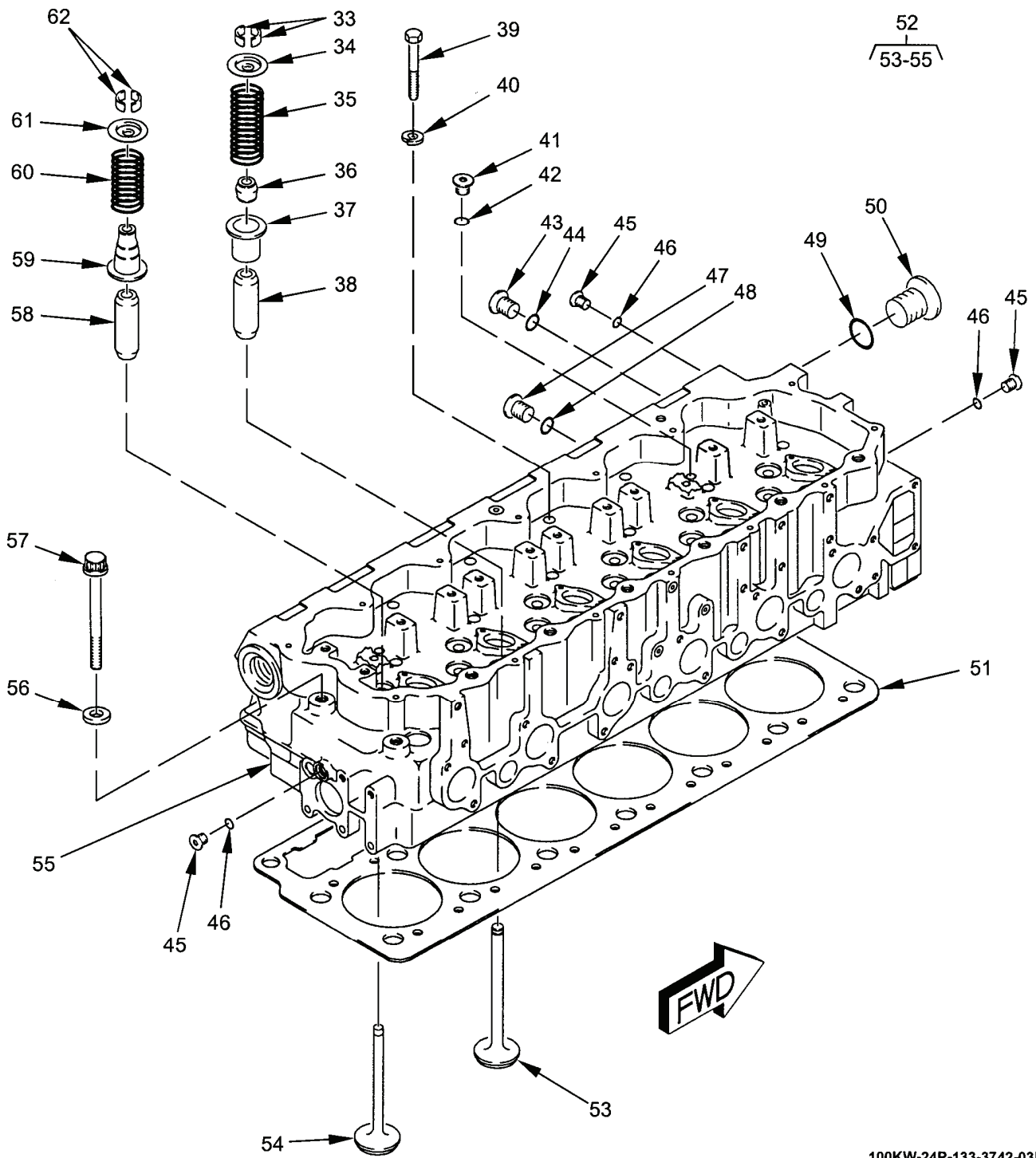
Figure 38. Cylinder Head Group (Sheet 3 of 3).
