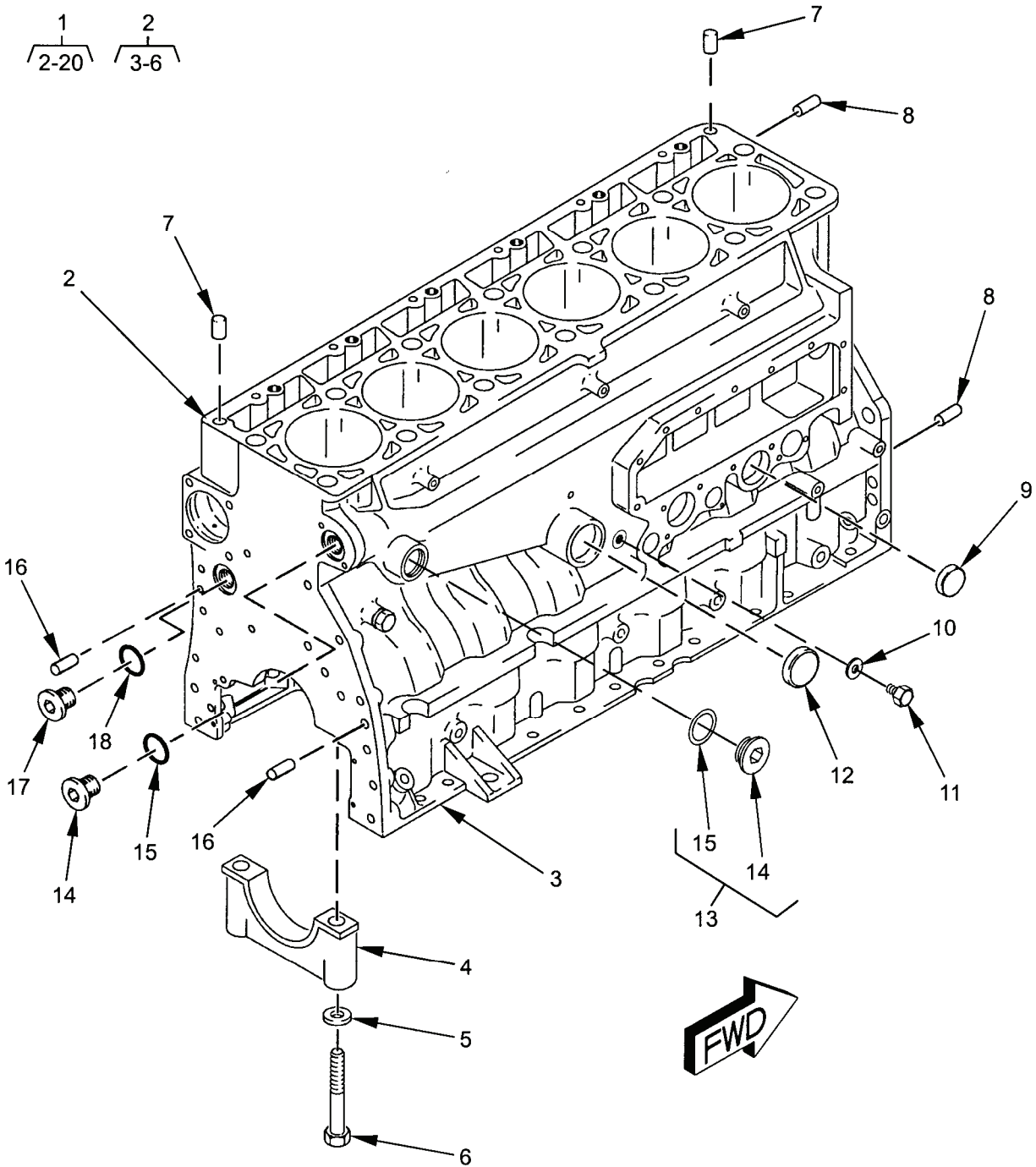
Figure 51. Cylinder Block Group (Sheet 1 of 2).
