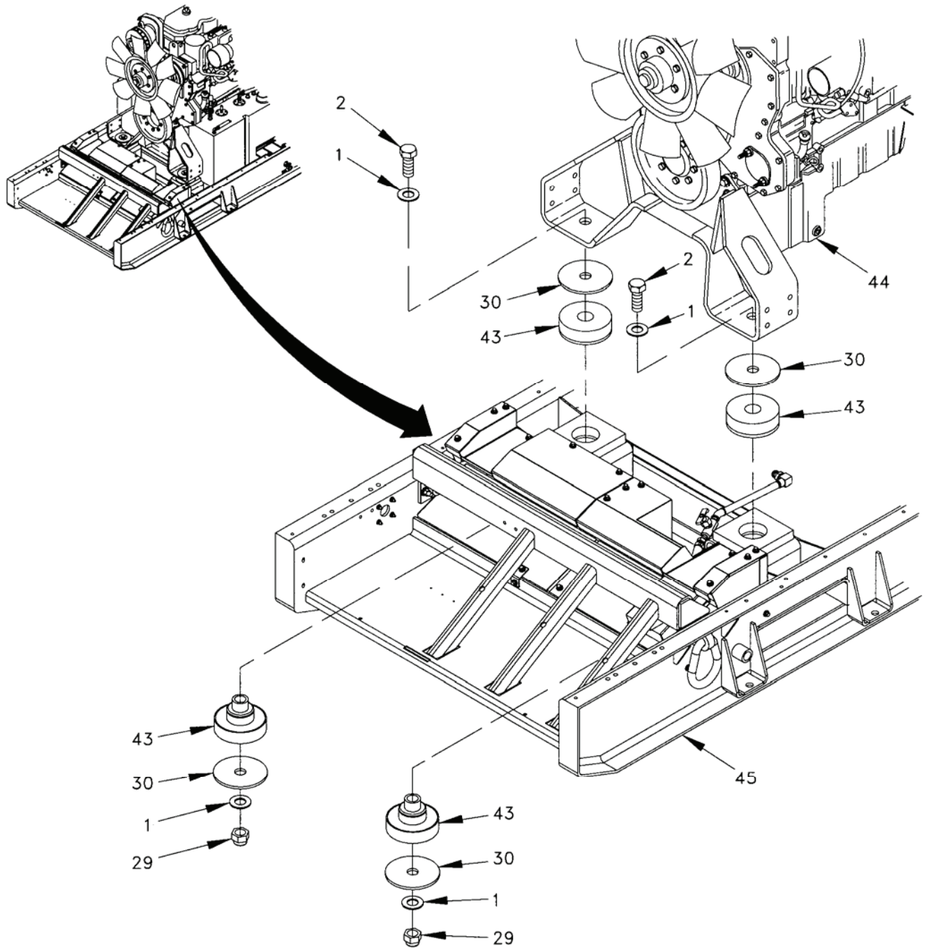
Figure 16. Engine Generator Base Assembly (Sheet 2 of 4).
