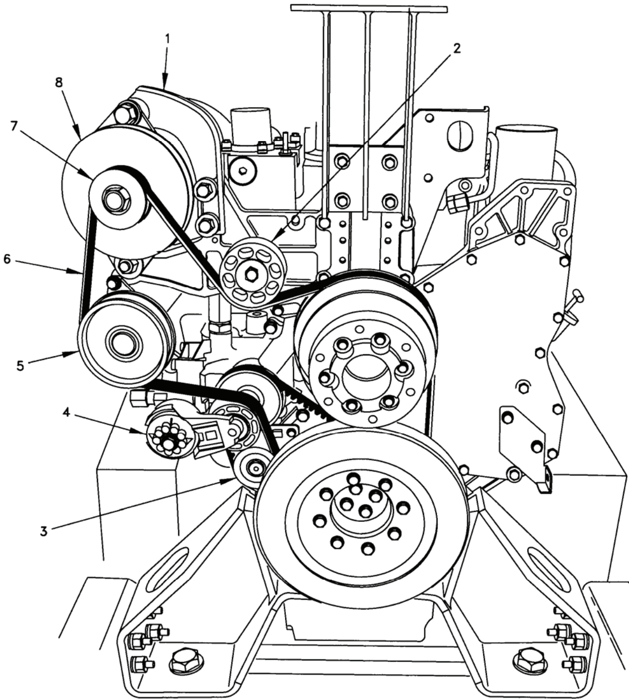
Figure 18. Engine Tensioner Group (Sheet 1 of 3).
