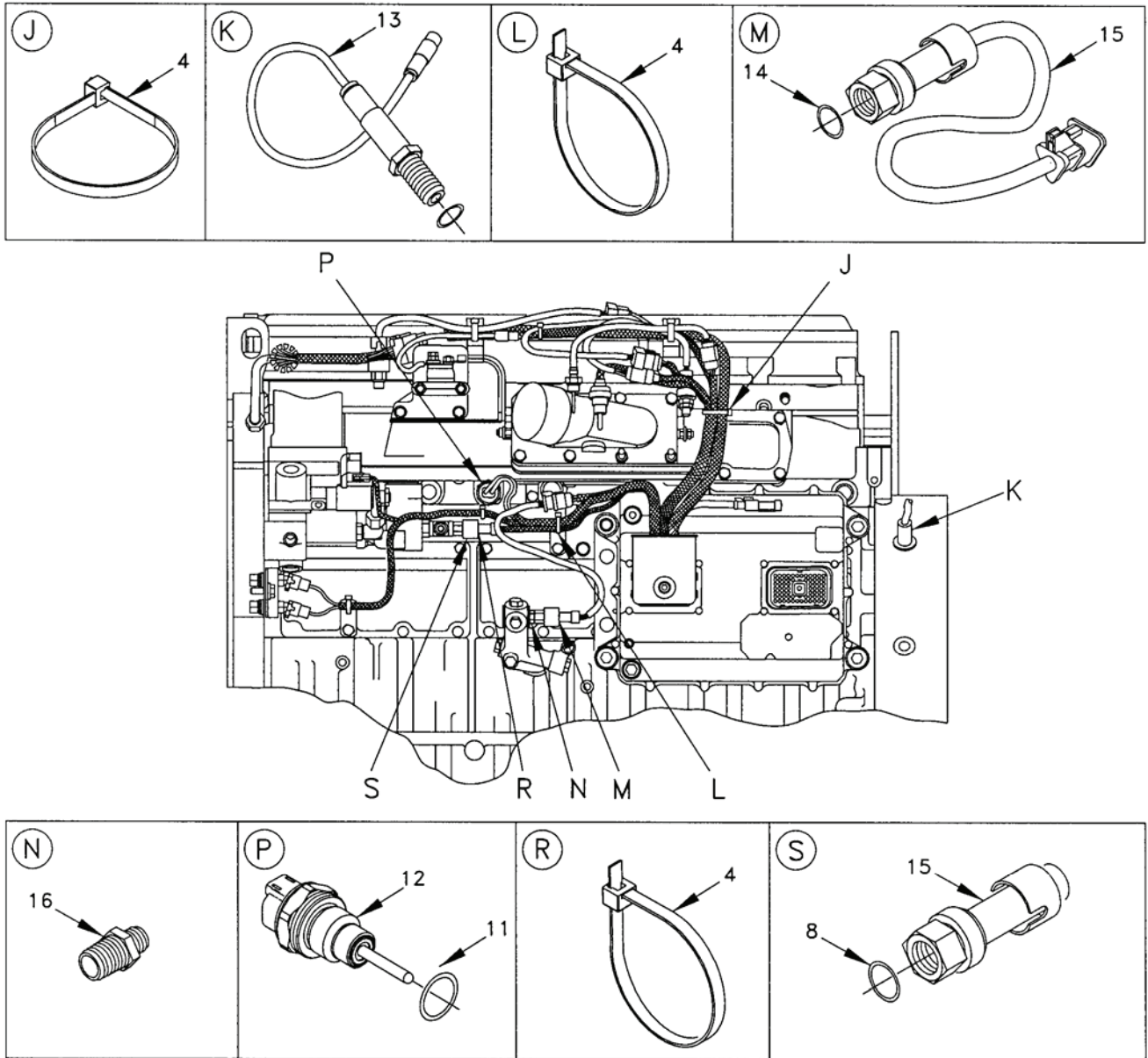
Figure 24. Sensor and Wiring Group (Sheet 2 of 4).
