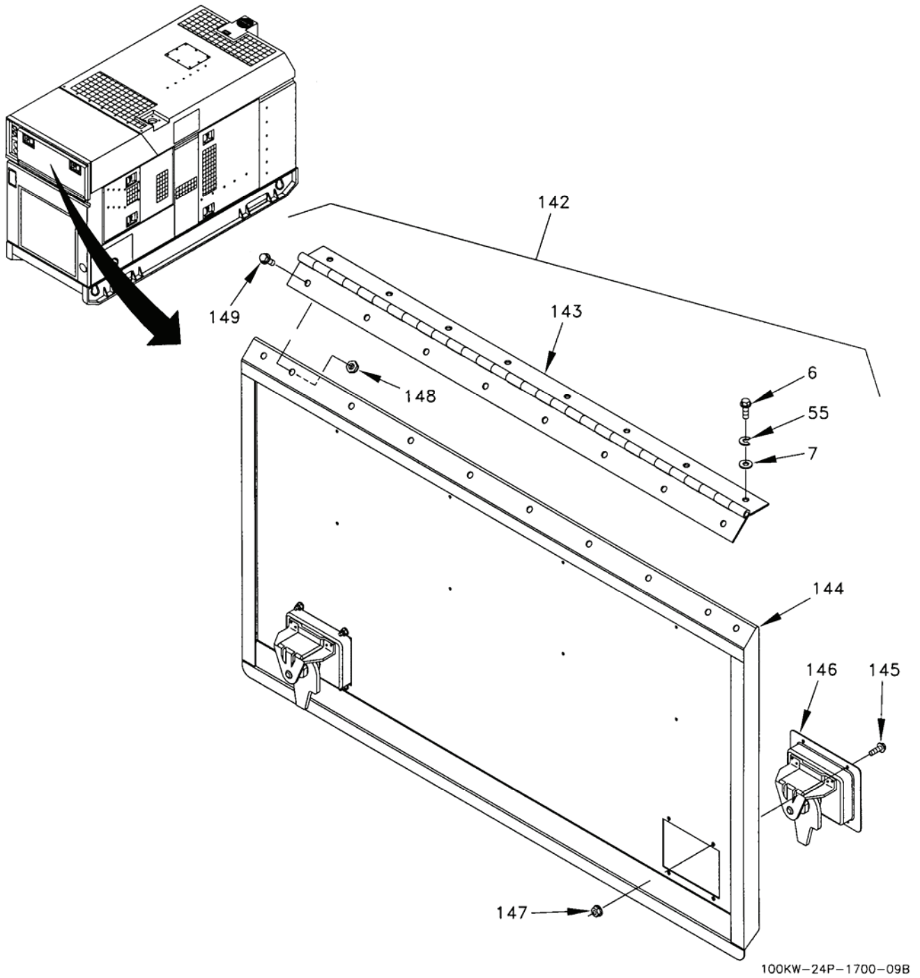
Figure 3. Housing Installation (Sheet 9 of 25).
