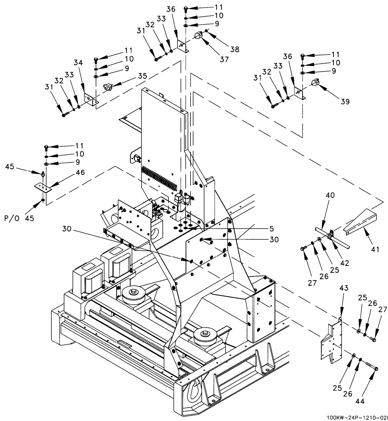
Figure 7. Electrical Components Installation (Sheet 2 of 8).
