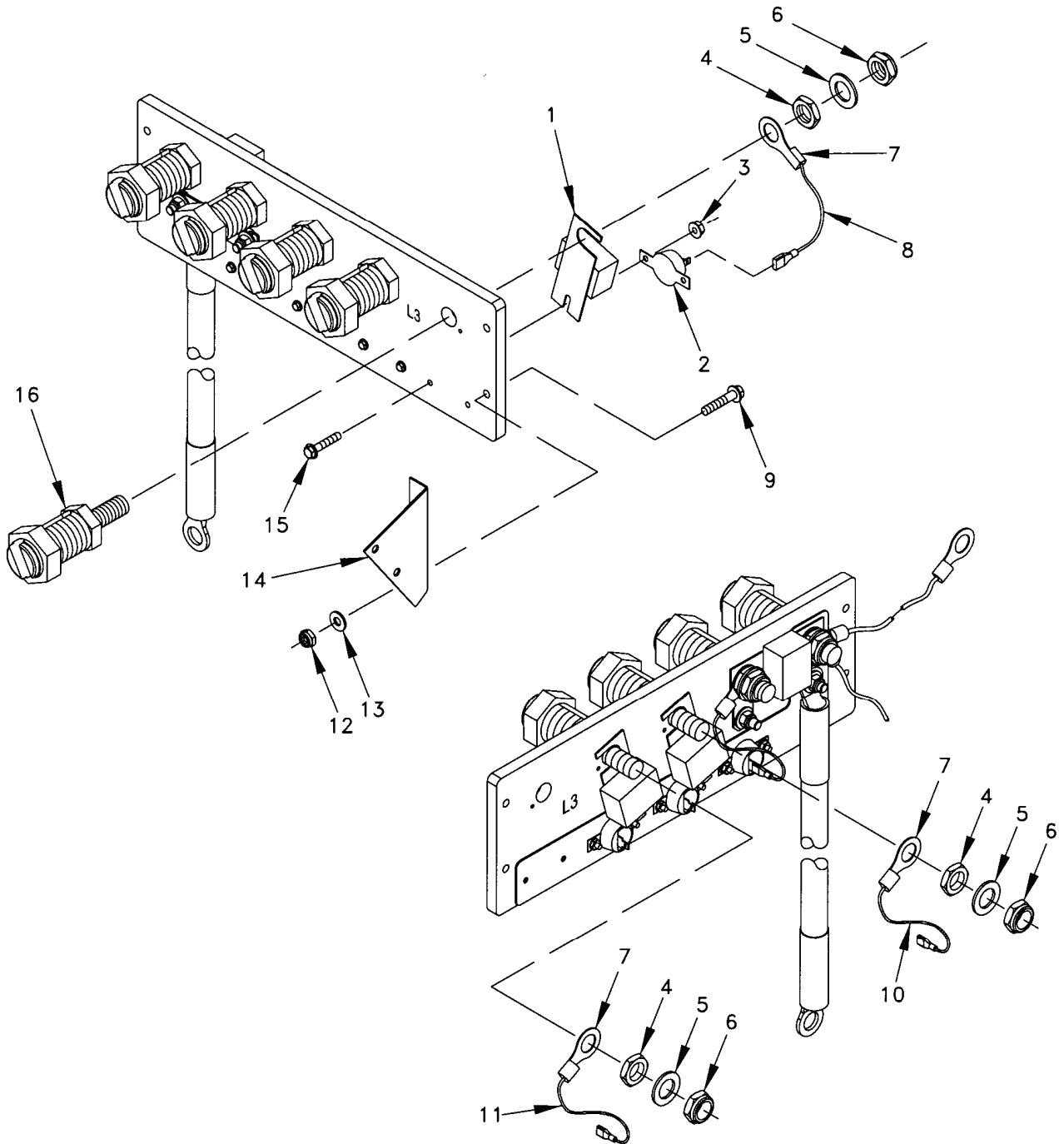
Figure 11. Load Terminal Board Assembly (Sheet 1 of 2).
