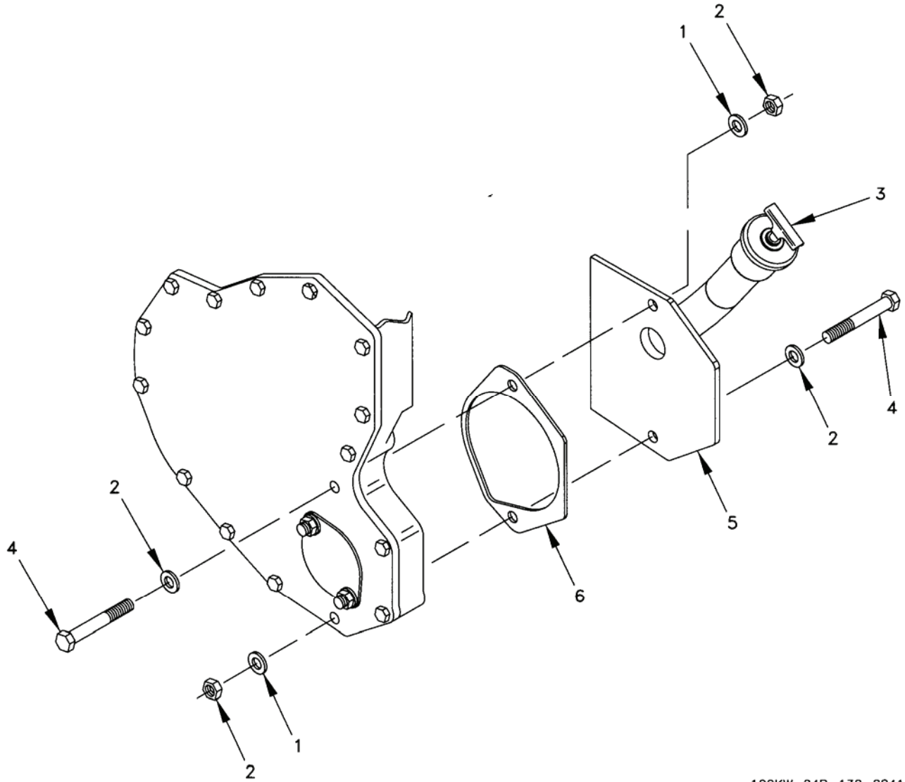
Figure 32. Oil Filler Group.
