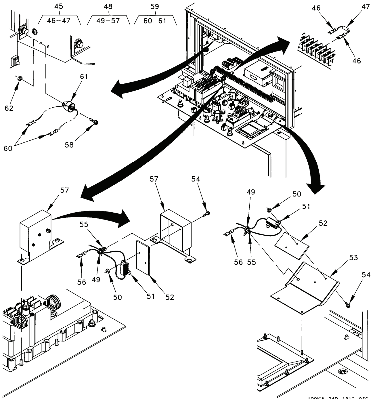
Figure 53. Winterization Kit Installation (Sheet 3 of 5).
