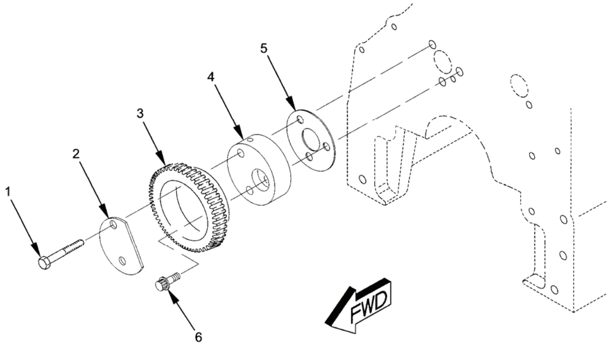
Figure 48. Front Gear Group.
