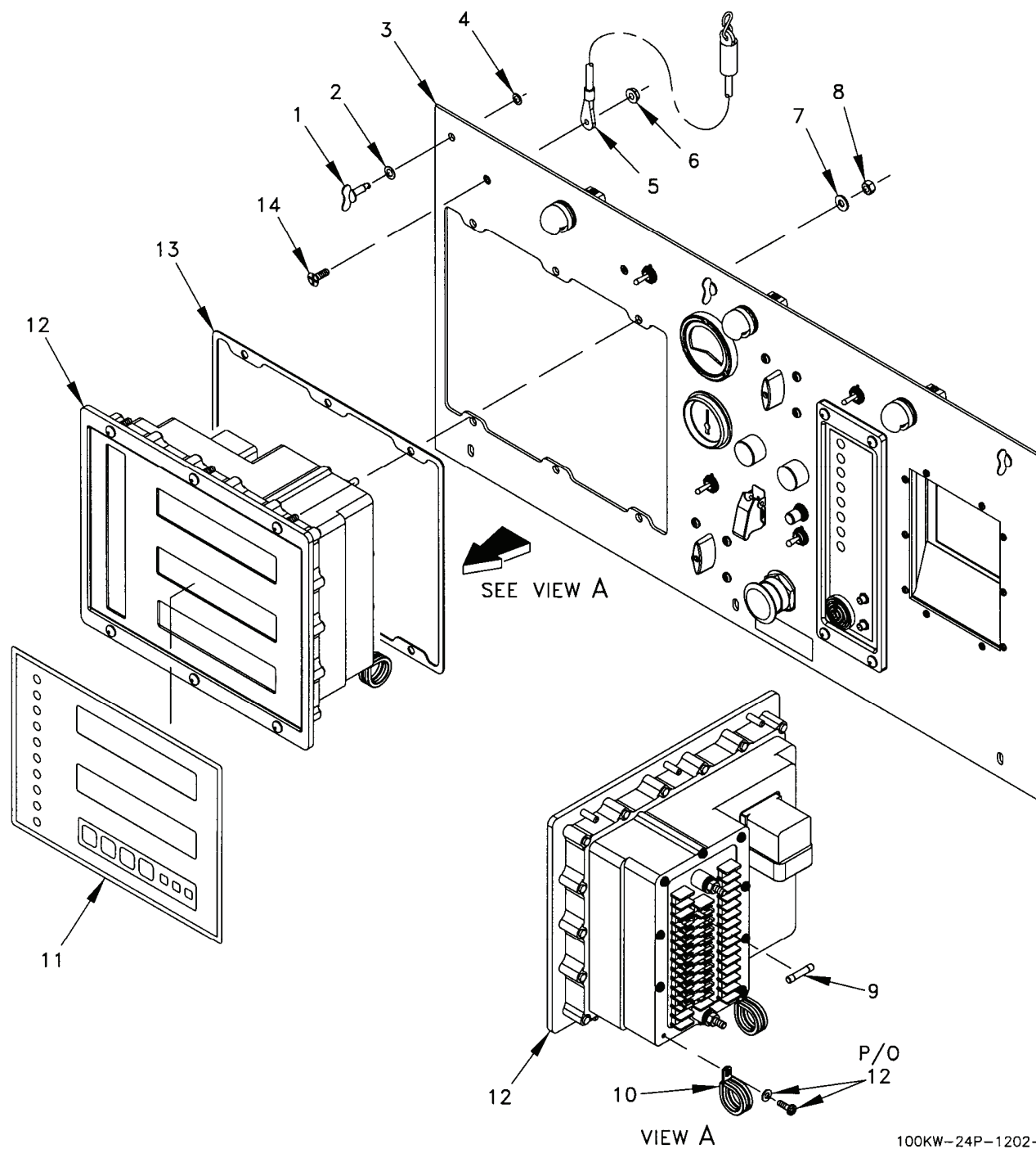
Figure 6. Control Box Panel Assembly (Sheet 1 of 3).
