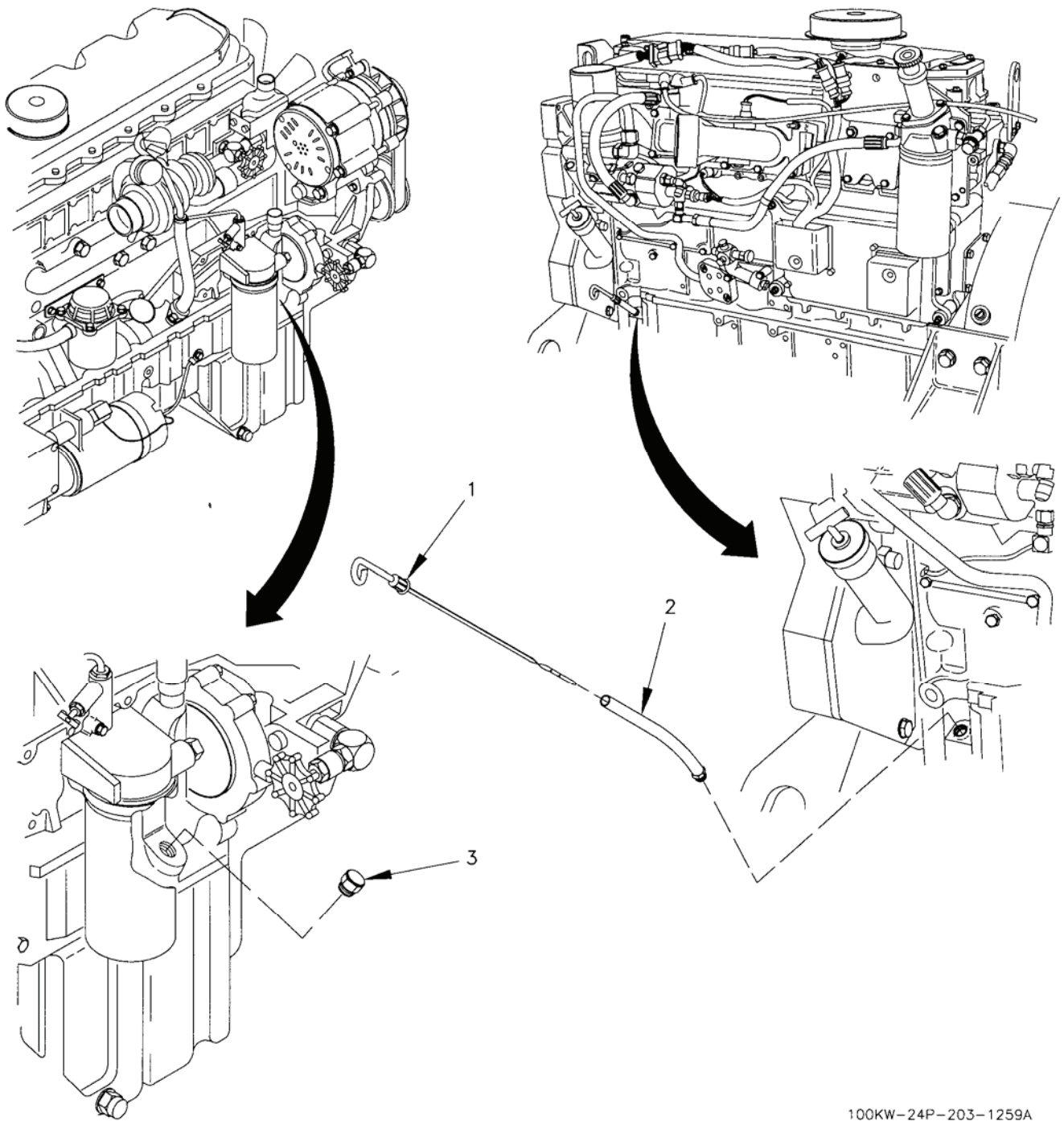
Figure 34. Oil Level Gage Group.
