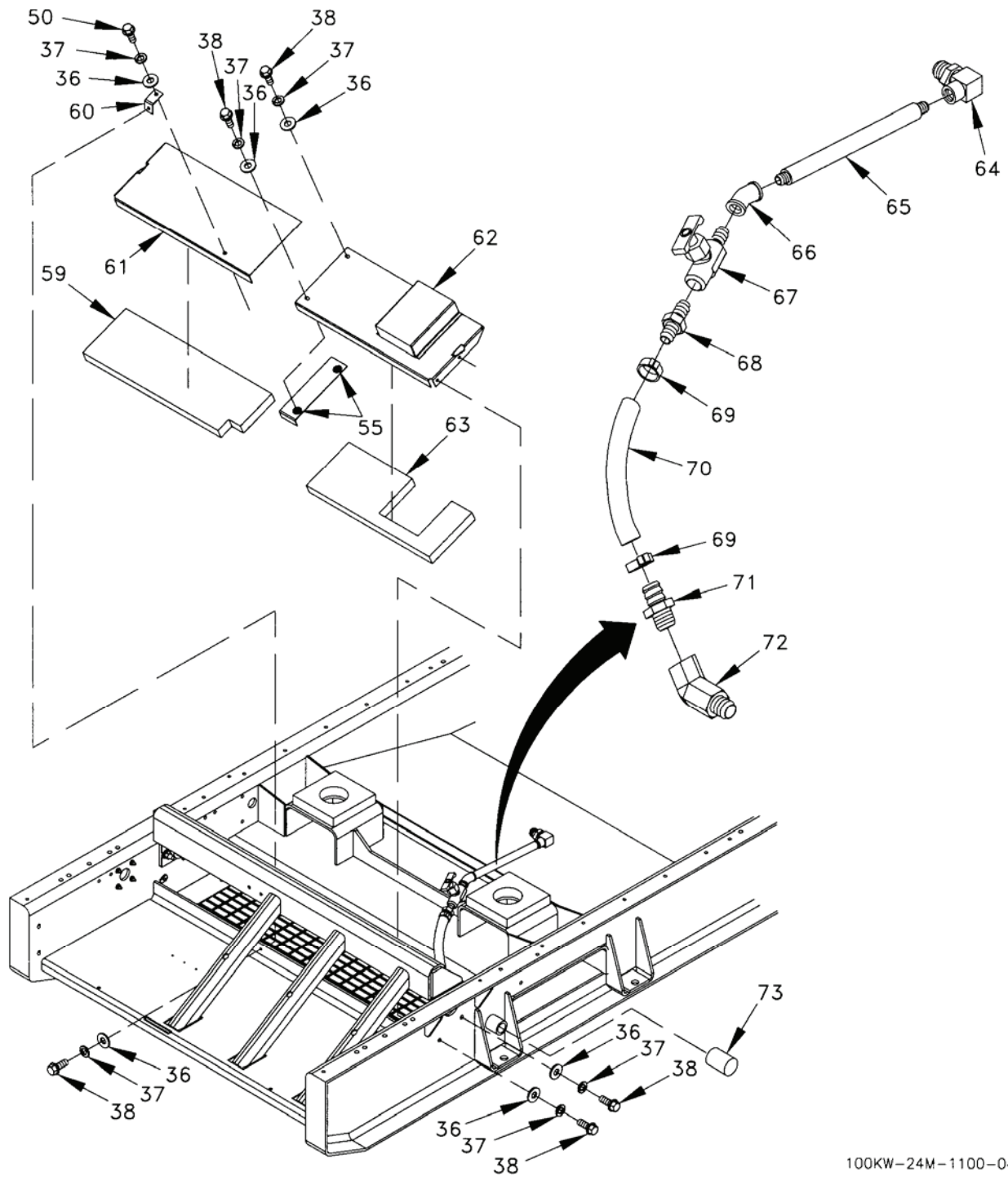
Figure 16. Engine Generator Base Assembly (Sheet 4 of 4).
