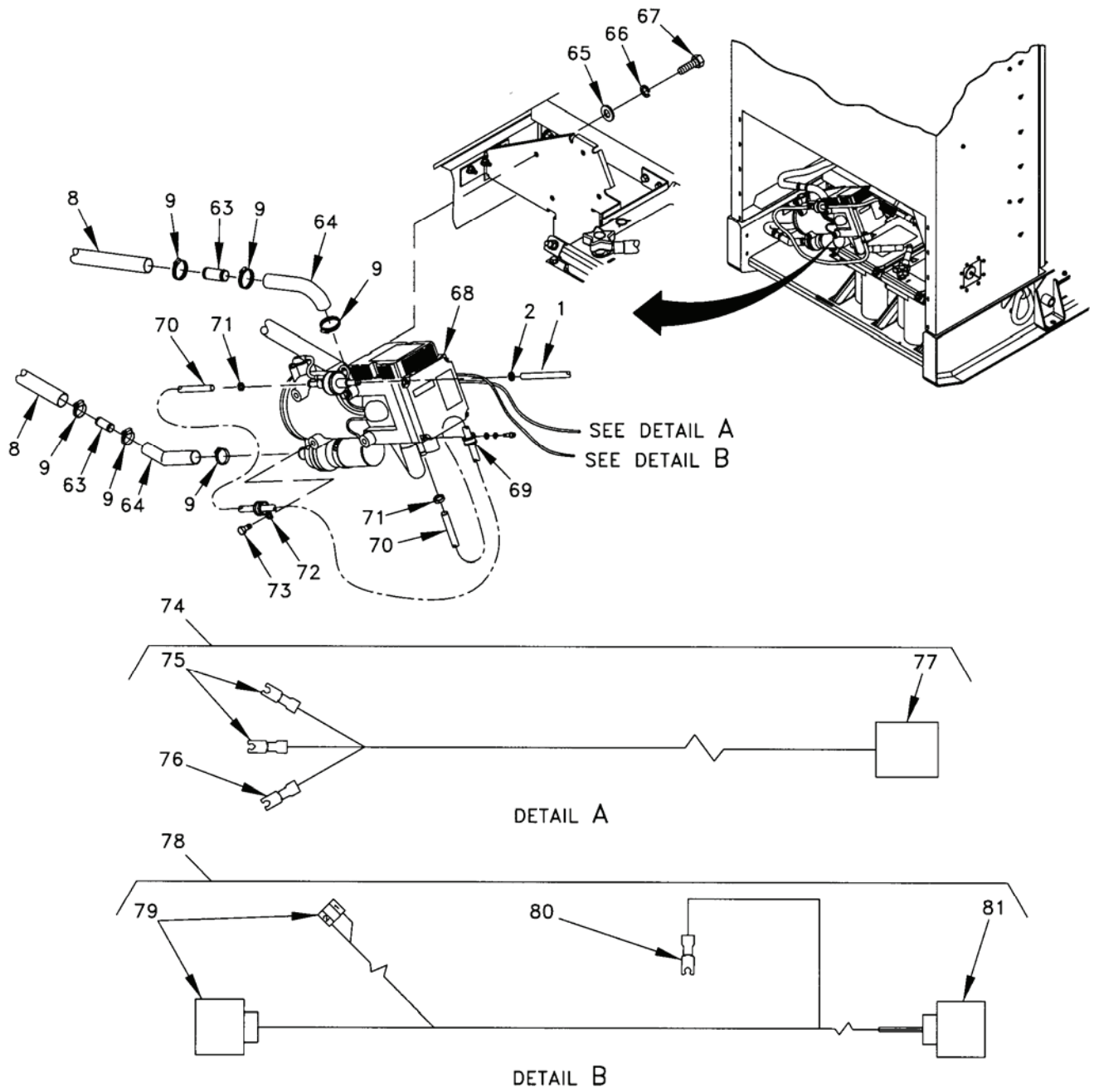
Figure 53. Winterization Kit Installation (Sheet 4 of 5).
