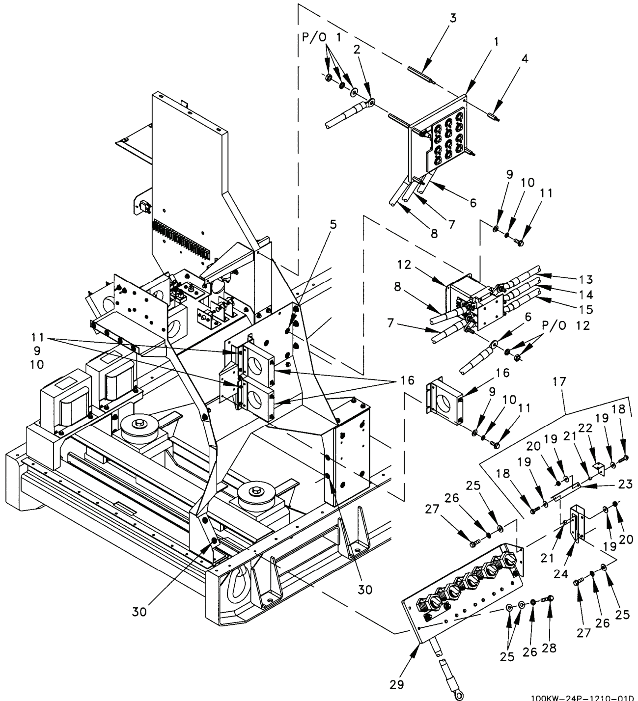
Figure 7. Electrical Components Installation (Sheet 1 of 8).
