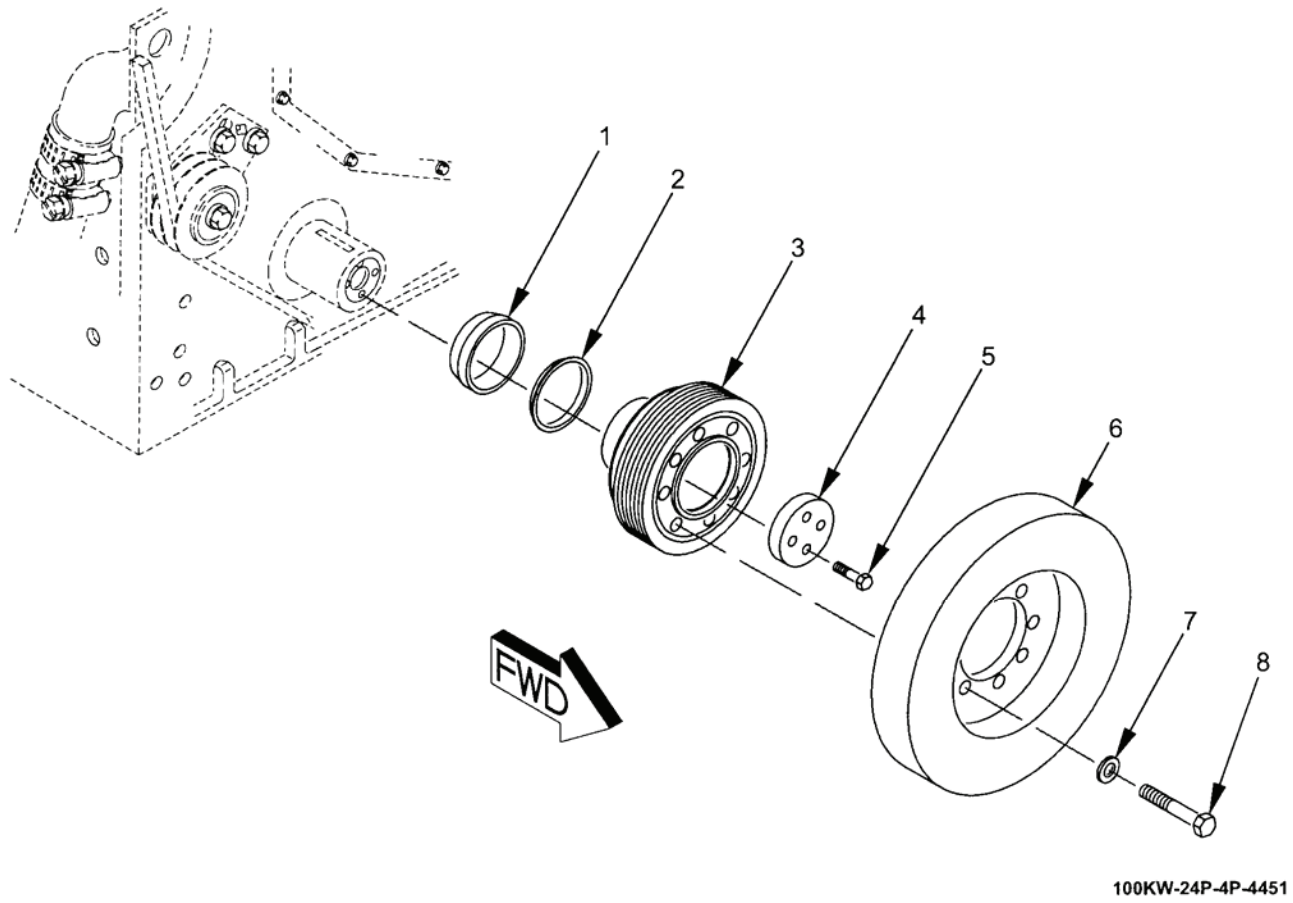
Figure 44. Crankshaft-Damper Group.
