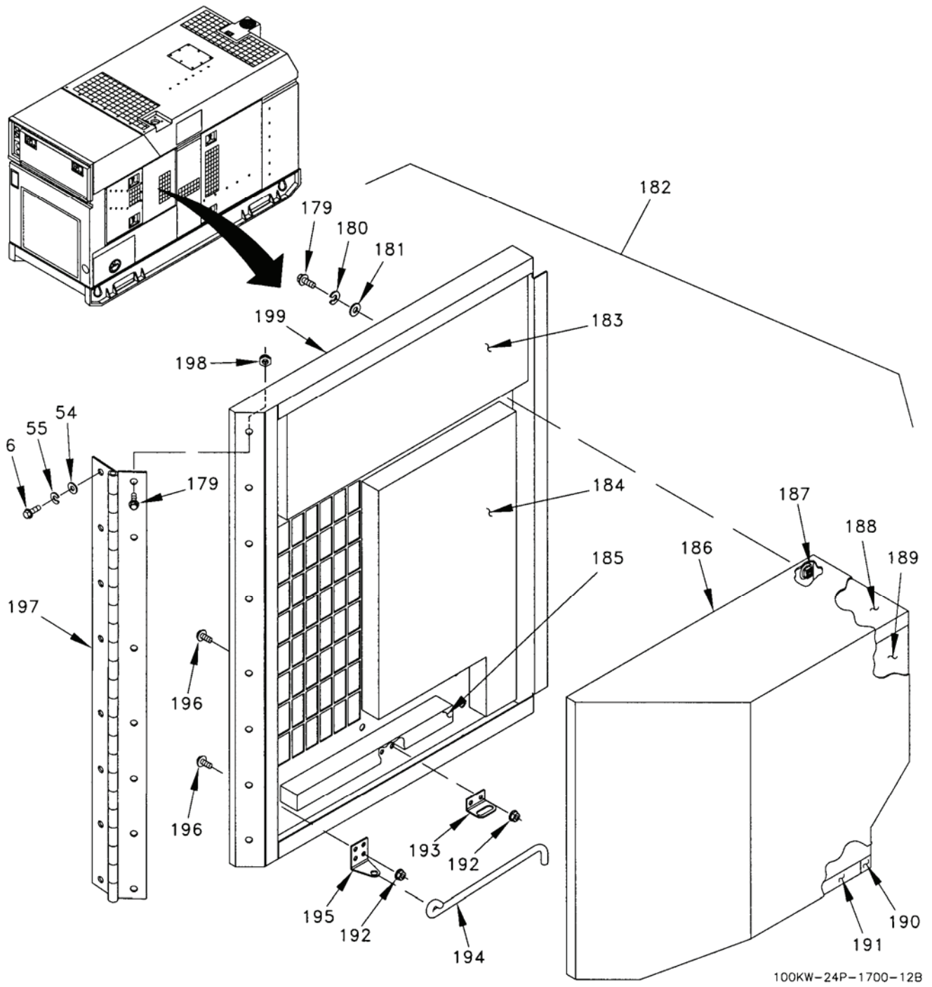
Figure 3. Housing Installation (Sheet 12 of 25).
