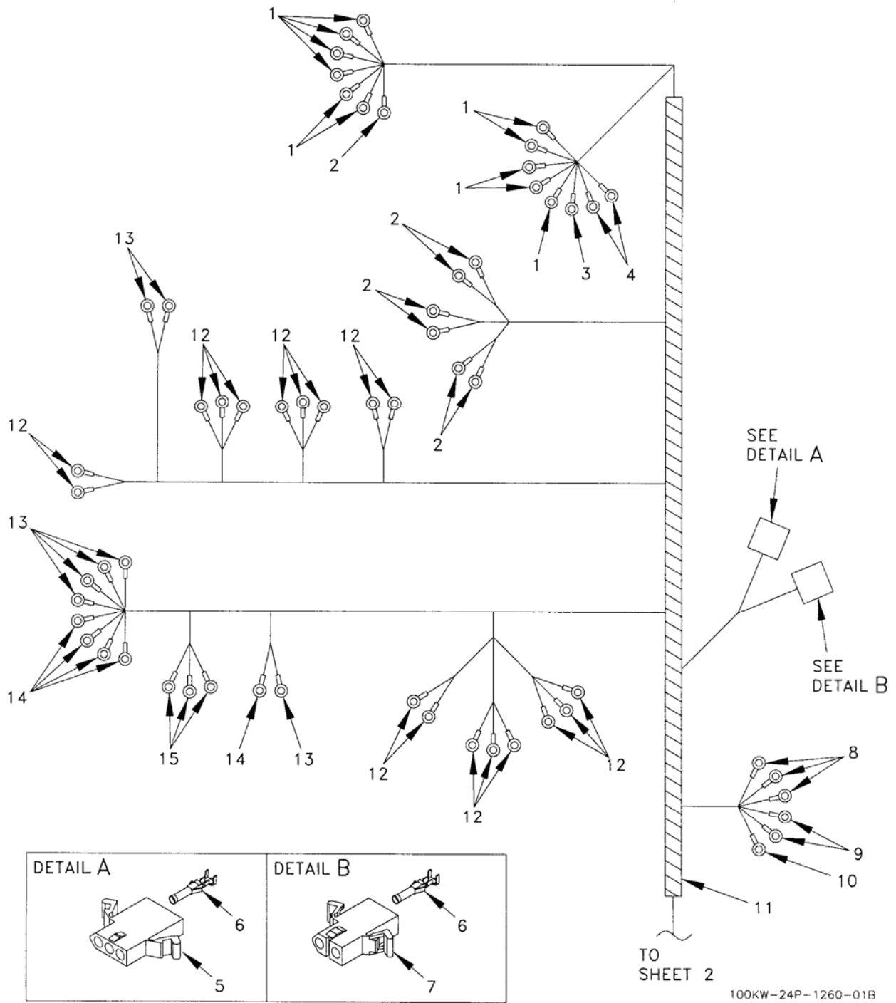
Figure 9. Engine Harness Assembly (Sheet 1 of 3).
