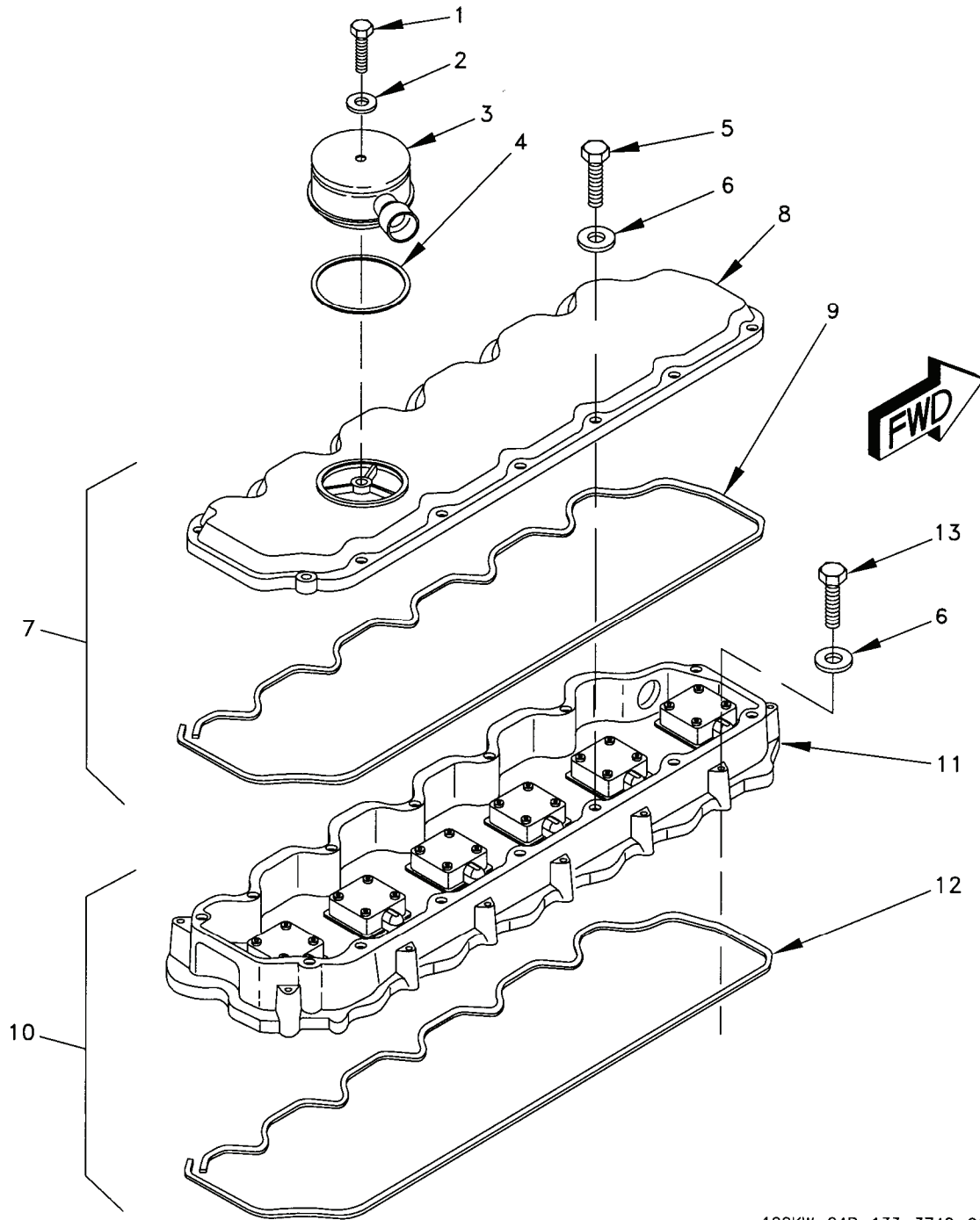
Figure 38. Cylinder Head Group (Sheet 1 of 3).
