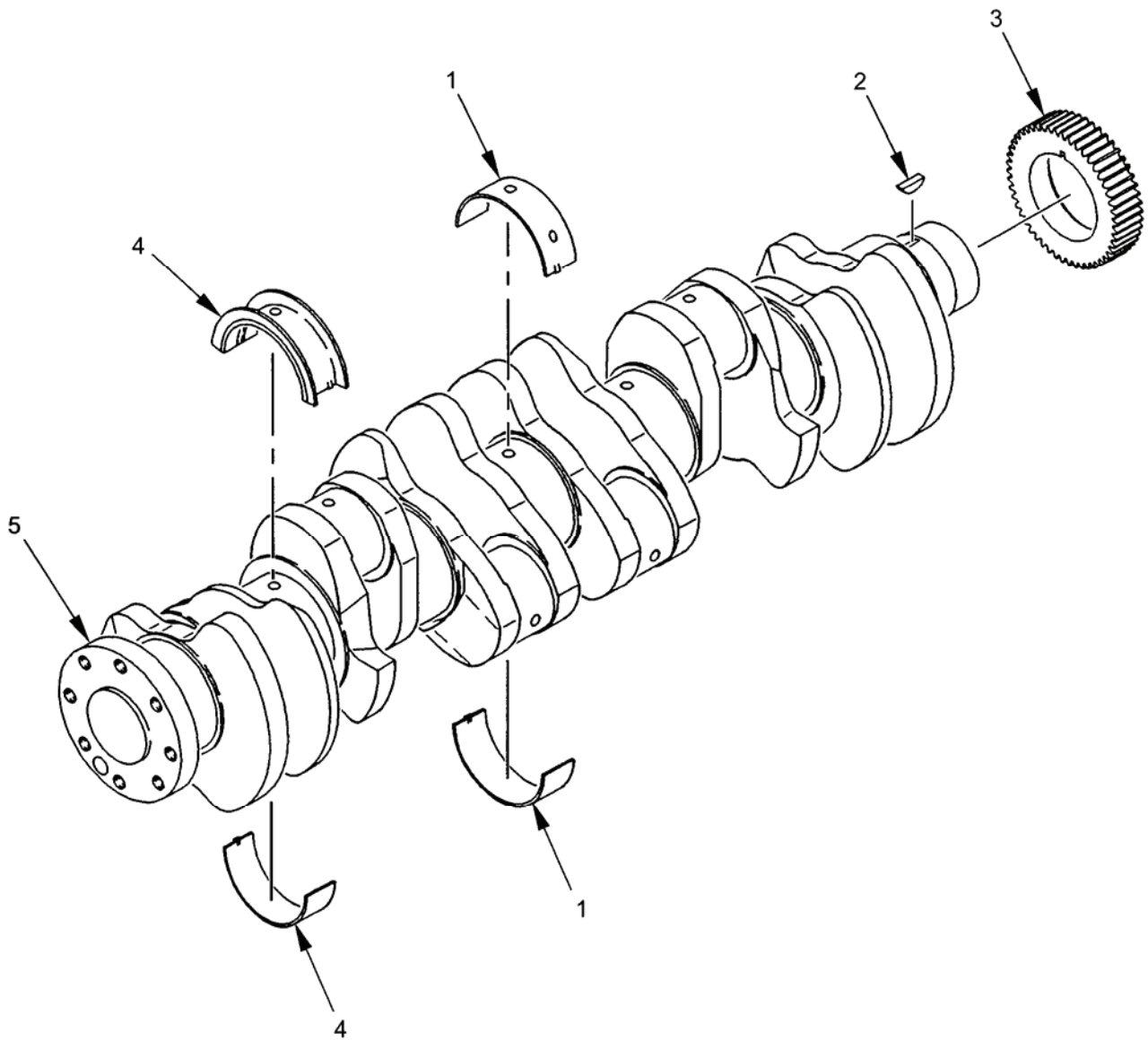
Figure 45. Crankshaft Group.
