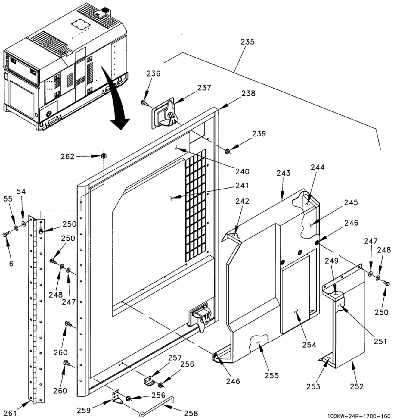
Figure 3. Housing Installation (Sheet 16 of 25).
