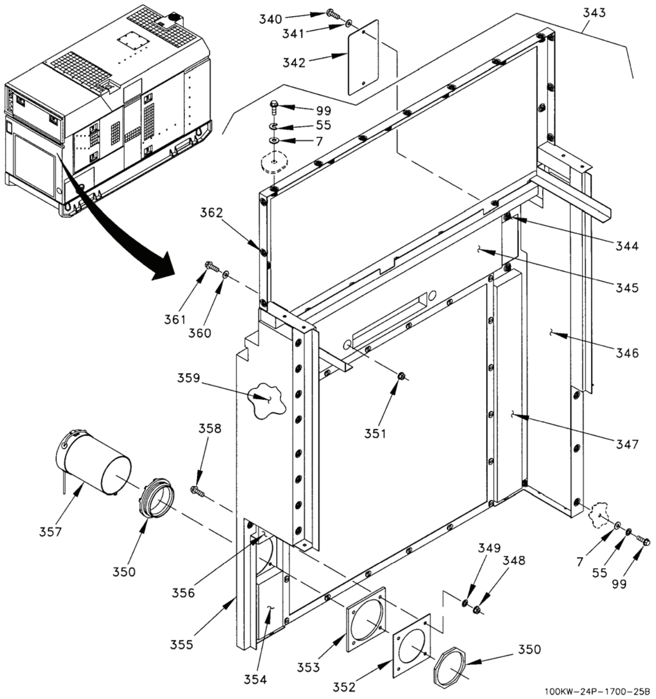
Figure 3. Housing Installation (Sheet 25 of 25).
