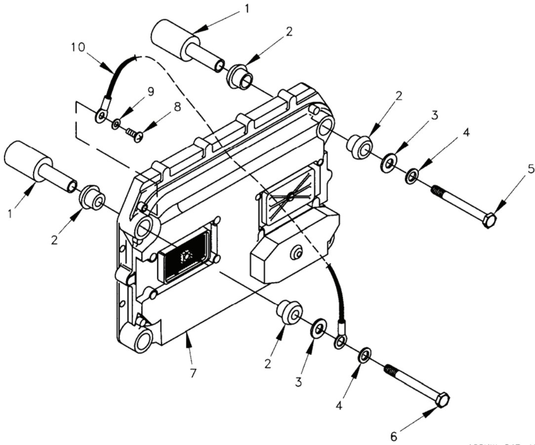
Figure 25. Controller Group.
