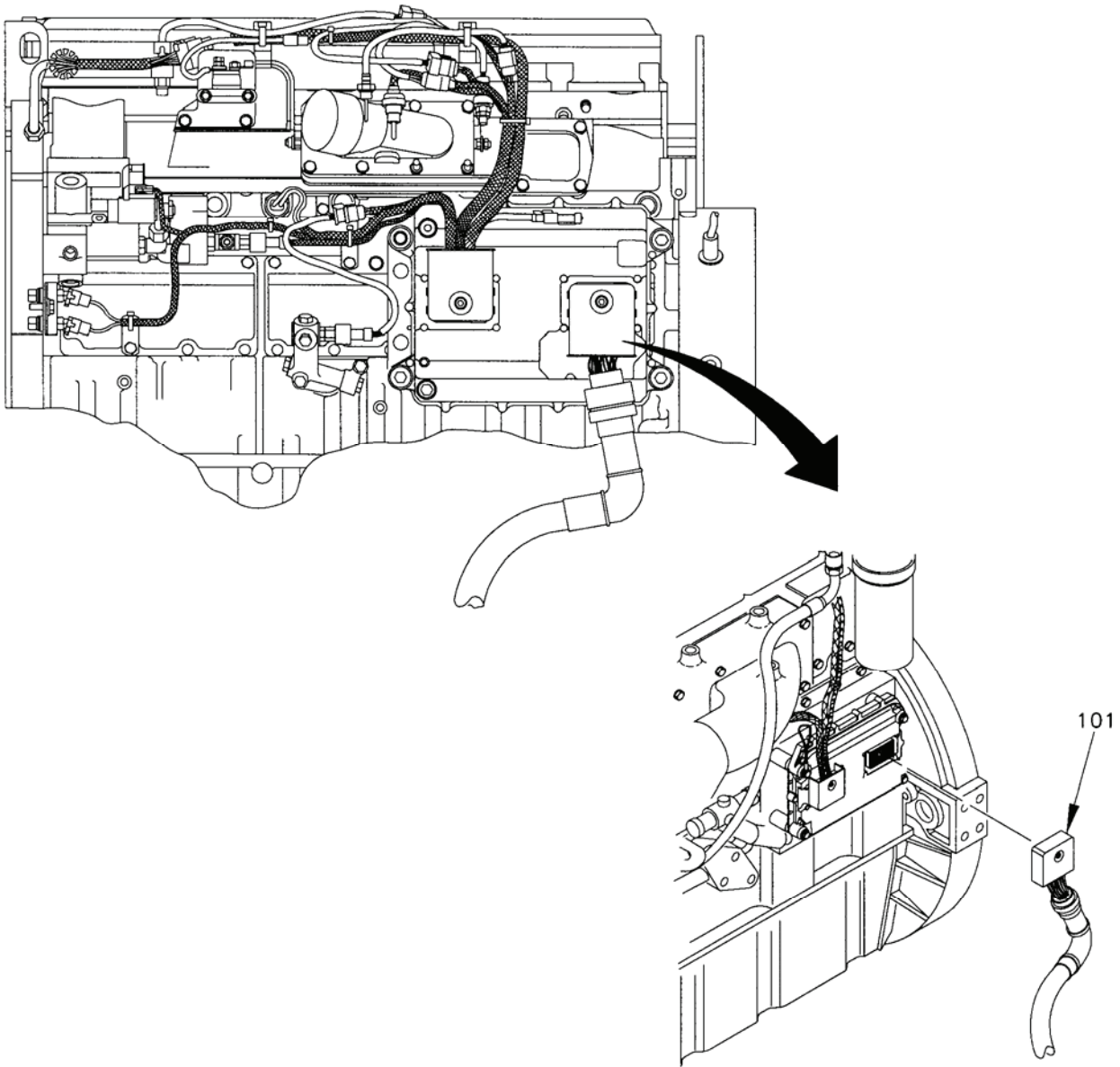
Figure 7. Electrical Components Installation (Sheet 8 of 8).
