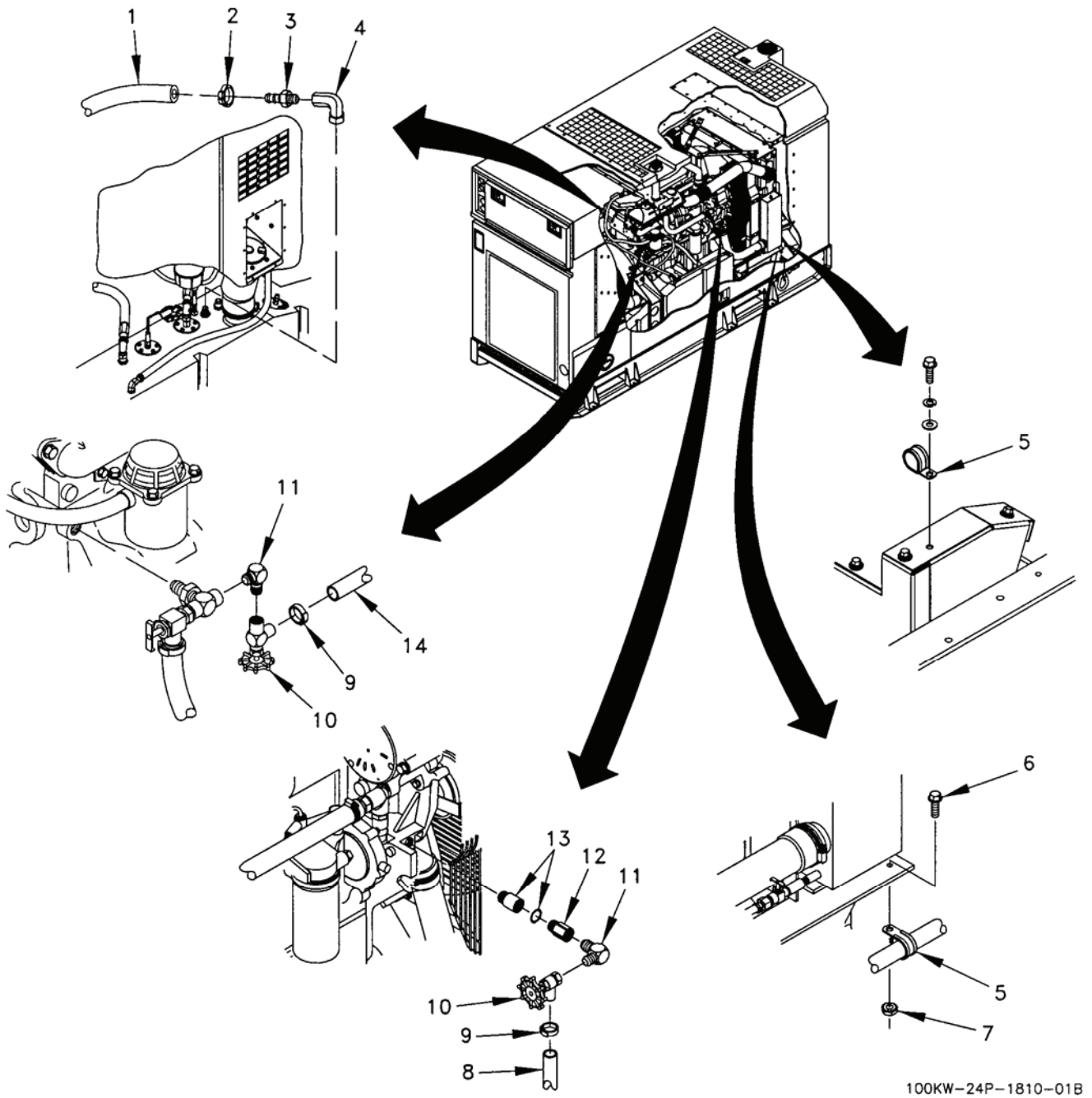
Figure 53. Winterization Kit Installation (Sheet 1 of 5).
