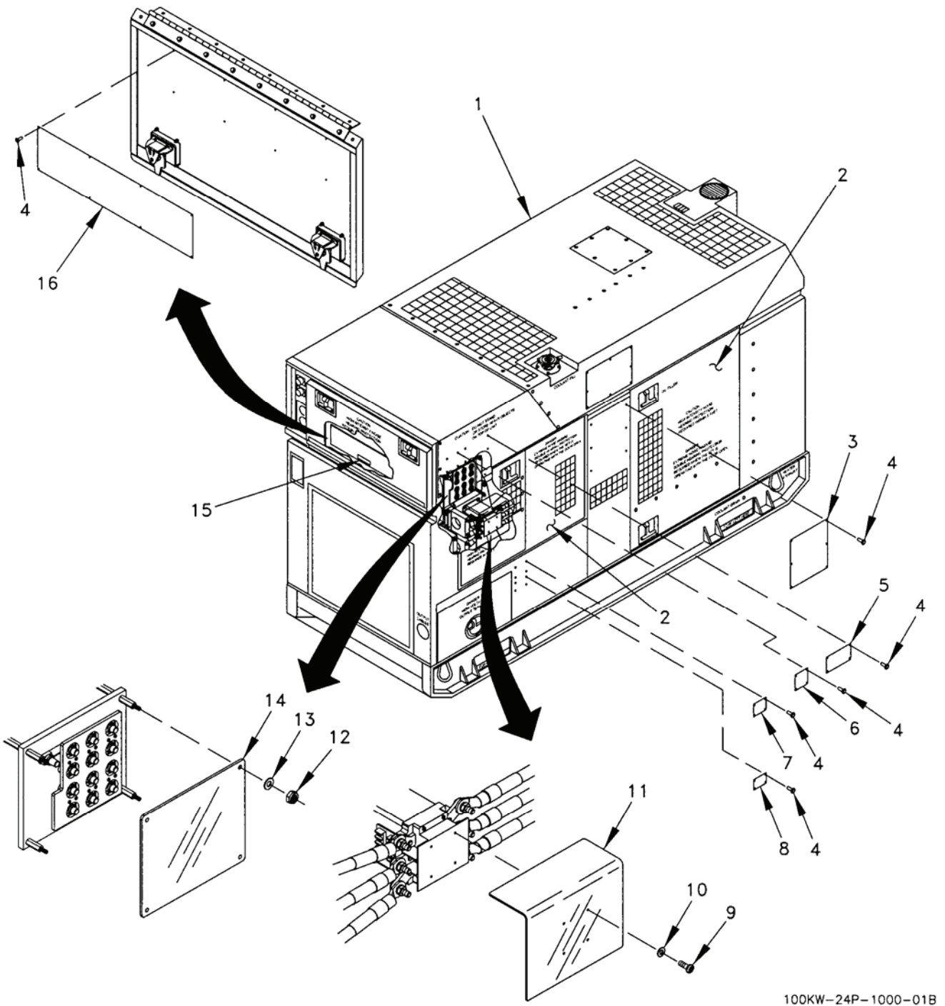
Figure 1. Generator Set, Tactical Quiet, 100 kW, 50/60 Hz (Sheet 1 of 3).
