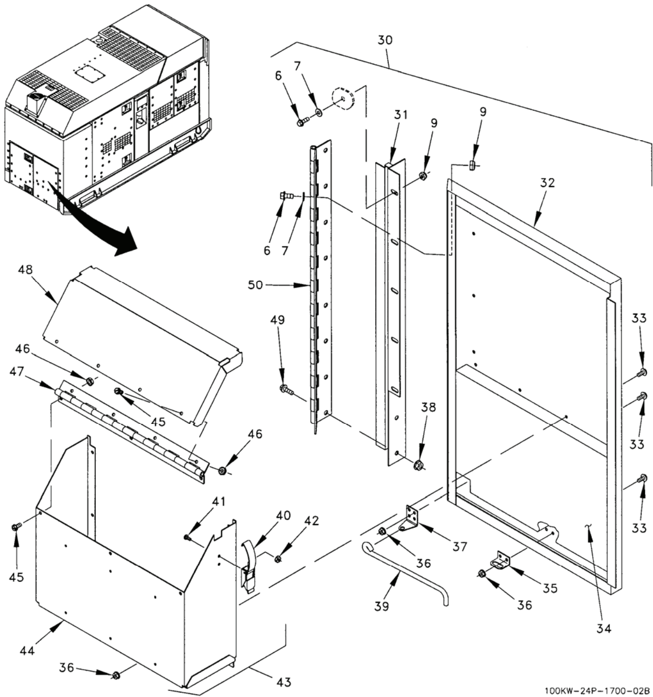
Figure 3. Housing Installation (Sheet 2 of 25).
