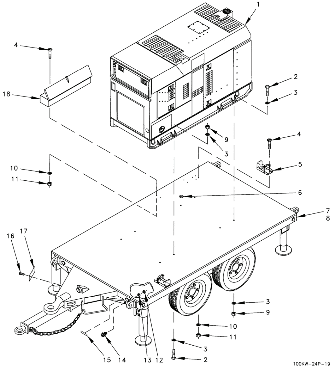
Figure 54. Trailer Installation.
